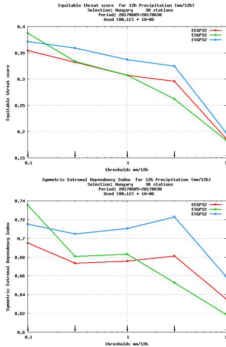
Figure 10. The ETS and SEDI scores of +12 hour precipitation (12-hour accumulation) as a function of precipitation thresholds. Scores are visualized for experiments EEGPS2 (red), ESGPS2 (green) and EVGPS2 (blue). Verification period between 5th and 30th of June 2017, Data selection: Hungary, 30 stations
