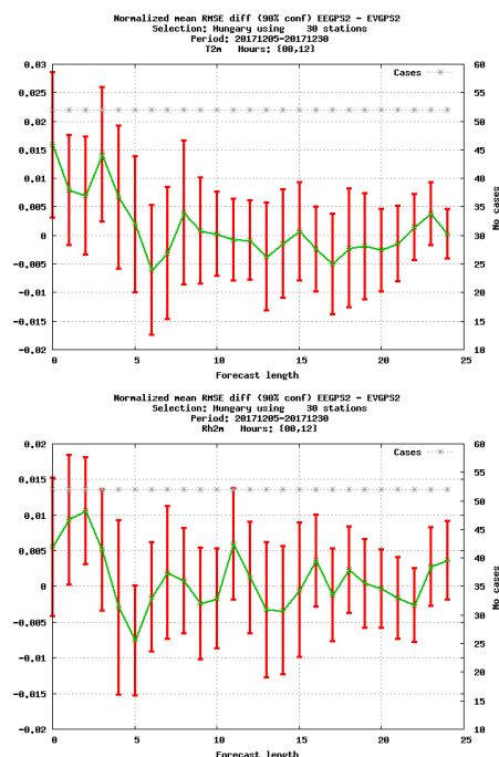
Figure 11. The Normalized RMSE difference of screen-level temperature (K) and relative humidity (%) as a function of forecast range. Scores are comparing EEGPS2 and EVGPS2 experiment. Verification period between 5th and 30th of December 2017, Data selection: Hungary
