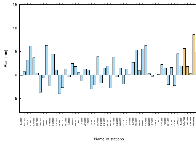
Figure 5. The BIAS in mm for SGO1 (light blue) and WUEL (light orange) networks calculated for the period of 15-31st of May, 2017
