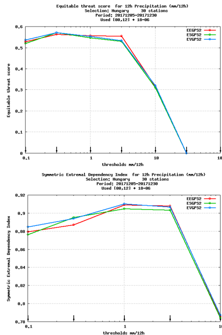
Figure 12. The ETS and SEDI scores of +12 hours precipitation (12-hour cummulation) as a function of precipitation thresholds. Scores are visualized for experiments EEGPS2 (red), ESGPS2 (green) and EVGPS2 (blue). Verification period between 5th and 30th of December 2017, Data selection: Hungary
