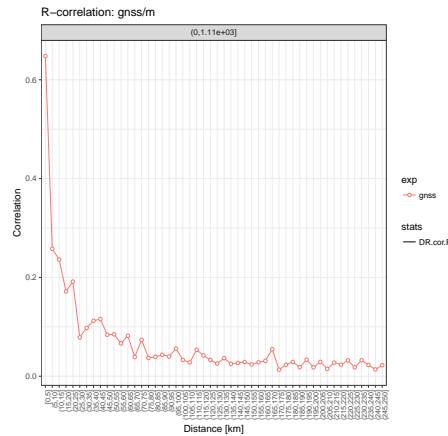
Figure 3. Observation error correlations estimated by Desroziers method as a function of separating distances for GNSS ZTDs
