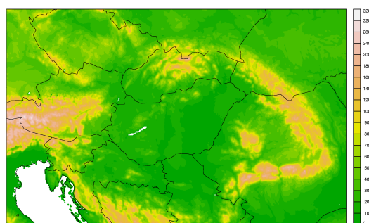
Figure 1. The computational domain of AROME/Hungary
