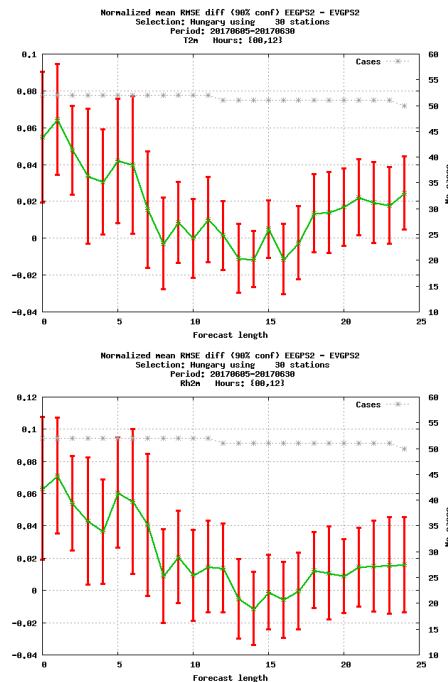
Figure 8. The Normalized RMSE difference of screen-level temperature (K) and relative humidity (%) as a function of forecast range. Scores are comparing EEGPS2 and EVGPS2 experiment. Verification period between 5th and 30th of June 2017, Data selection: Hungary
