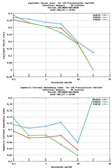
Figure 9. The ETS and SEDI scores of +12 hours precipitation (12-hour cummulation) as a function of precipitation thresholds. Scores are visualized for experiments EEGPS2 (red), ESGPS2 (green) and EVGPS2 (blue). Verification period between 5th and 30th of June 2017, Data selection: Hungary
