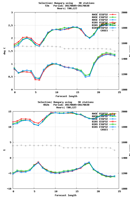
Figure 7. The RMSE and BIAS of screen-level temperature (K) and relative humidity (%) as a function of forecast range. Scores are plotted for EEGPS2 (red), ESGPS2 (green) and EVGPS2 (blue). Verification period between 5th and 30th of June 2017, Data selection: Hungary
