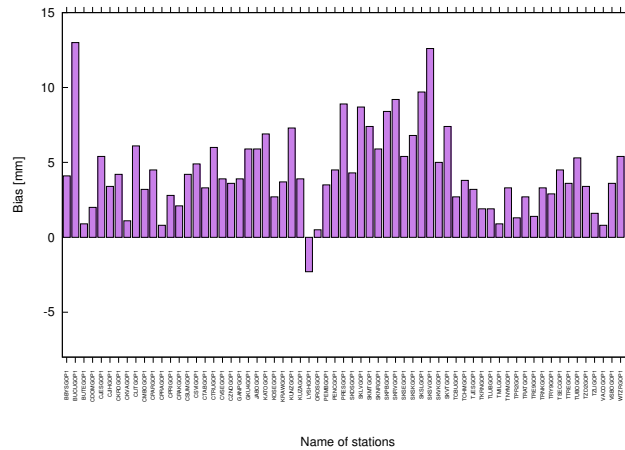
Figure 6. The BIAS in mm for GOP1 (purpule) network calculated for the period of 15-31st of May, 2017
