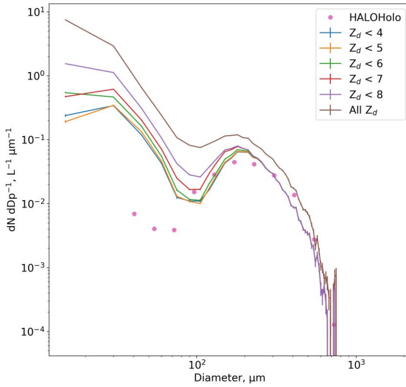
Figure 11a. Size distributions for a straight and level run at -42^{\circ}\text{C} in cirrus (16:02:00 to 16:10:00, 7 February) from a holographic imaging probe (pink markers) and the CIP-15 using different Z_d thresholds. Figure 10b shows example CIP-15 images from this period. Decreases in detector intensity of 25 to 50%, 50 to 75% and >75\% are shown as light blue, black and orange pixels, respectively. Vertical lines show the Poisson counting uncertainty, these are very small for most of the size spectrum apart from > 700\text{ }\mu\text{m} where they become visible.
