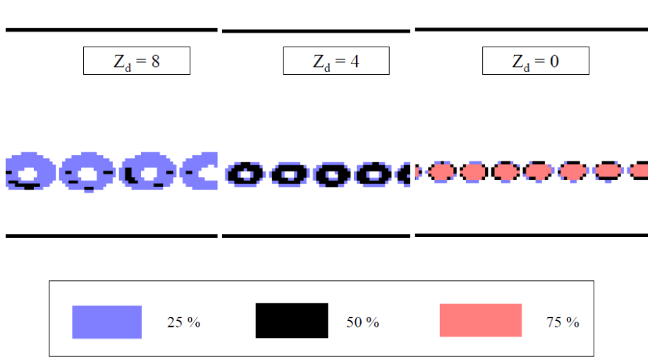
Figure 5. Example images from the CIP-15 of droplets from the droplet generator using a 90 μm printhead at Z_d = 8 (left), Z_d = 4 (middle) and Z_d = 0 (right). Decreases in detector intensity of 25 to 50%, 50 to 75% and >75% are shown as light blue, black and orange pixels, respectively.
