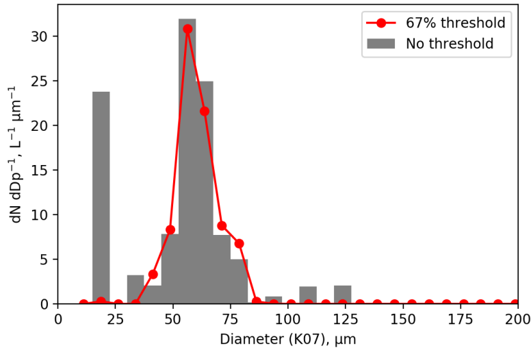
13 14 Figure 6. Size distribution of the K07 corrected diameter for a drop generator scan using the 15 60 \mu\text{m} printhead. The grey bars show data from all droplets, while the red markers show only 16 images with at least one pixel with a >67% decrease in detector intensity. This reduces the 17 depth of field to Z_d < 4.8 .
