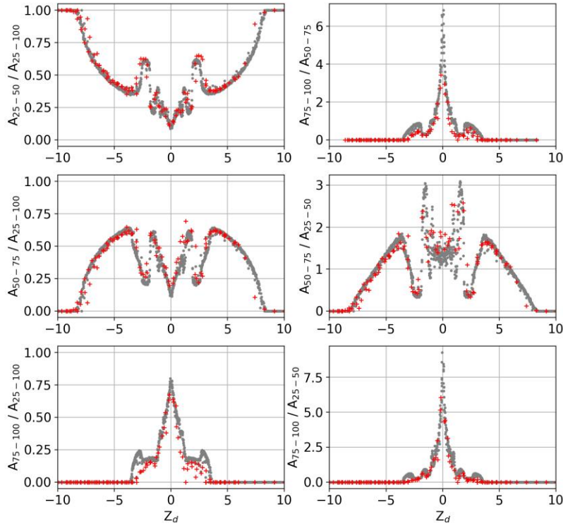
1 2 Figure 7. The ratios of the number of pixels between different thresholds from the drop 3 generator experiments (red) and model simulations of particles in the size range 50 to 150 \mu\text{m} 4 (grey) as a function of normalised distance from the object plane ( Z_d ).
