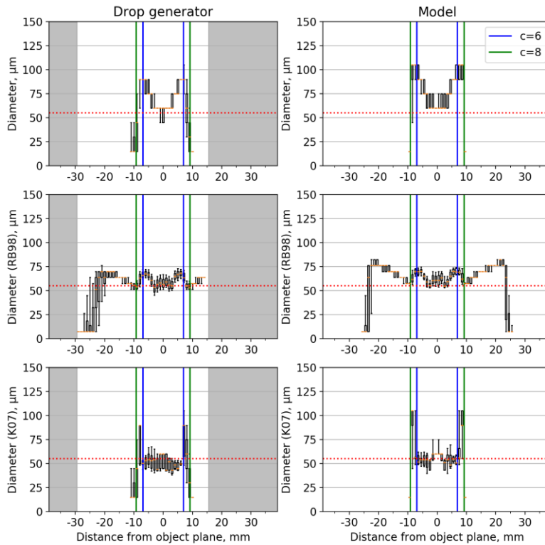
5 6 Figure 2. Box and whisker plots showing image diameter as a function of distance from the 7 object plane. Orange markers are the median diameter, boxes are the 25 and 75 th percentiles 8 and the whiskers are the 10 and 90 th percentiles. Left panels show results from the laboratory 9 experiments using a 60 \mu\text{m} pinhead. The grey shaded regions were not sampled using the 10 drop generator. Right panels show the model image diameter from a 55 \mu\text{m} particle. Top panels 11 show the image diameter using a 50% decrease in intensity threshold ( D_{50} ). Middle panels show
