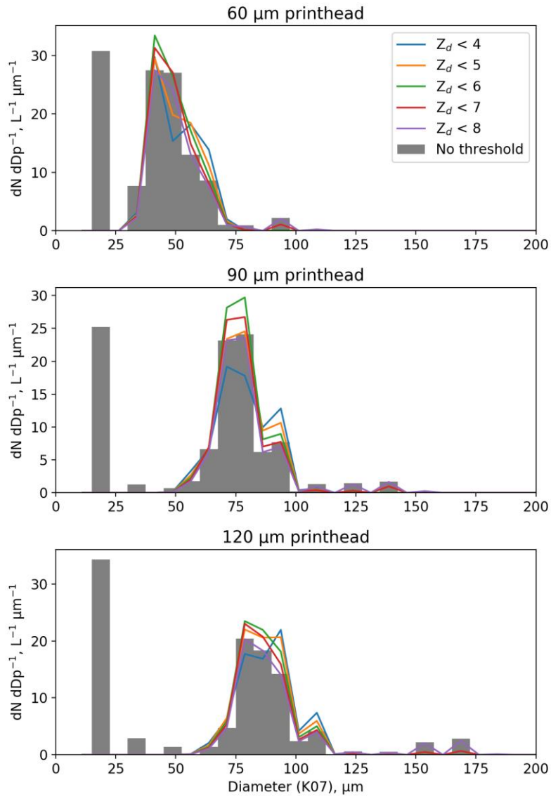
1 2 Figure 9. Size distributions of the K07 corrected diameter for drop generator scans of the CIP- 3 15 using the 60 \mu\text{m} (top panel), 90 \mu\text{m} (middle panel) and 120 \mu\text{m} (bottom panel) printheads. 4 The grey bars show data from all droplets, while the coloured lines show size distributions that
