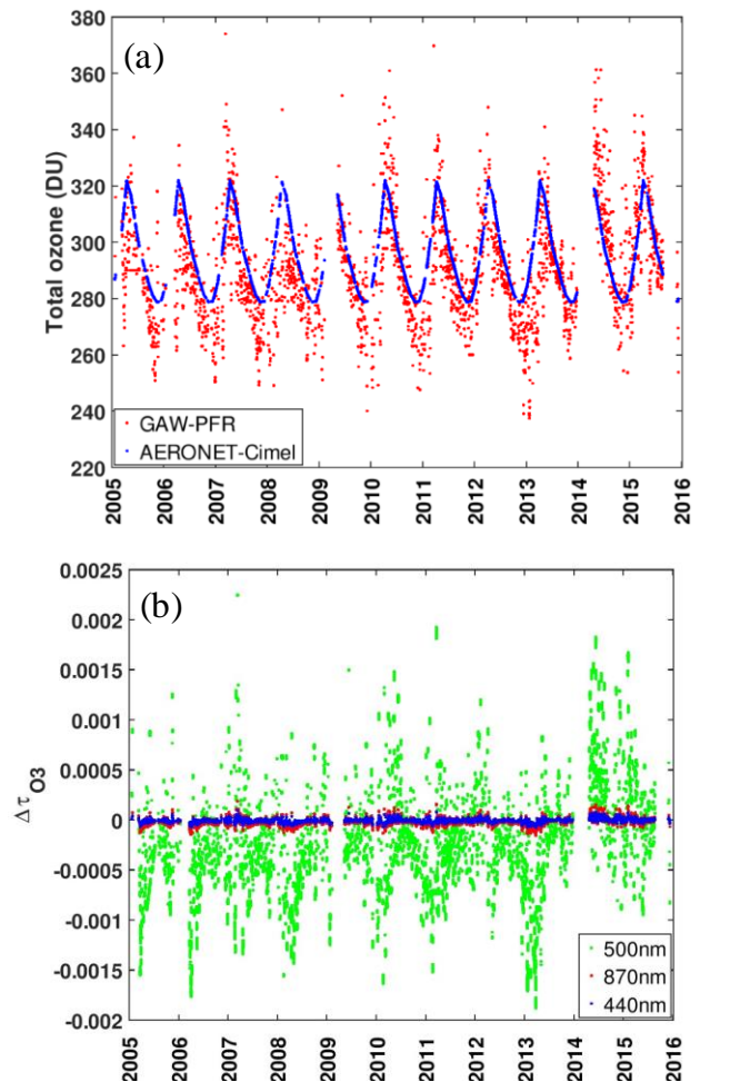
Figure 5. (a) Total O_3 used by GAW-PFR (measured Brewer O_3 values from IZO, OMI O_3 overpass or Brewer O_3 climatology) and AERONET-Cimel (TOMS O_3 climatology), and (b) \Delta\tau_{O_3}(\lambda) caused by differences in daily total O_3 between the two instruments in the period 2005-2015.
