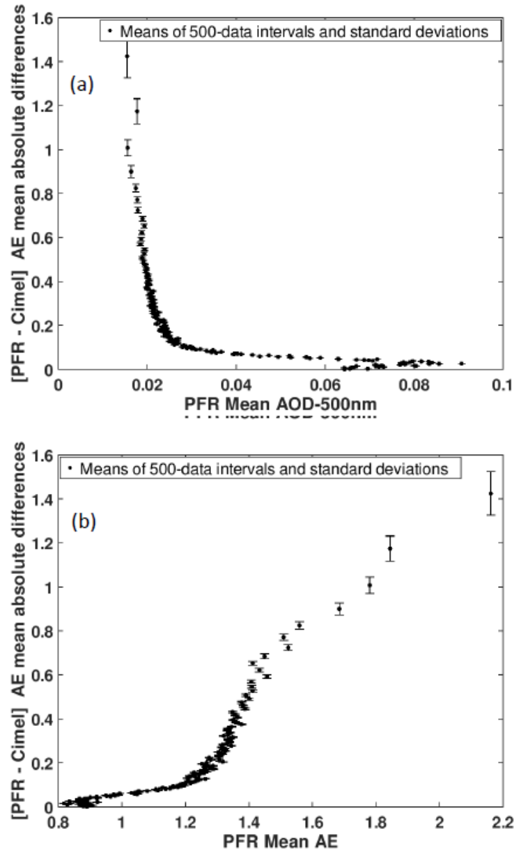
Figure 10. (a) PFR-Cimel AE mean absolute differences (and corresponding standard deviations) vs PFR mean AOD 500nm in 500 data intervals (b) and vs PFR mean AE in 500 data intervals. AE has been computed for both PFR and Cimel using the four common channels (380nm, 440nm, 500nm and 870nm).
