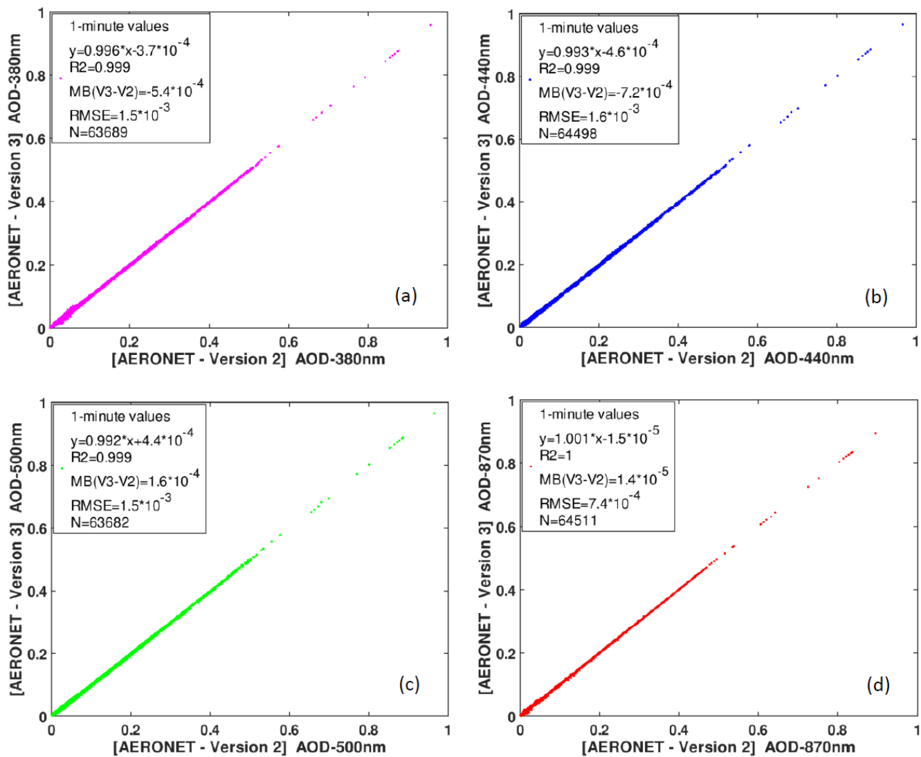
Figure 1. AERONET Version 3 (V3) vs Version 2 (V2) AOD 1-minute data scatterplot at Izaña Observatory for the period 2005-2015: (a) 380 nm; (b) 440 nm; (c) 500 nm and (d) 870 nm. The corresponding equations of the linear fits, the coefficients of determination ( R^2 ), Mean Bias (MB), Root Mean Square Error (RMSE) and the number of data pairs (N) used are included in each legend.
