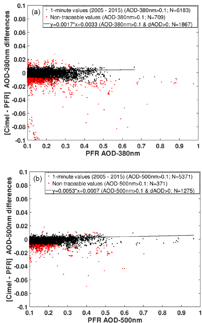
Figure 9. The same as Figure 7 after “correcting” the PFR AOD data by adding + 3.3 % at 380nm and + 2.2 % at 500 nm to the 1-minute PFR AOD data > 0.1.
