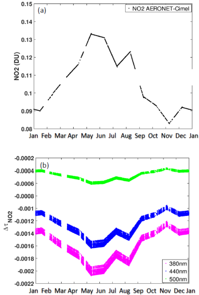
Figure 6. (a) NO 2 monthly climatology obtained from the ESA SCanning Imaging Absorption SpectroMeter for Atmospheric CHartographyY (SCIAMACHY), used by AERONET-Cimel at IZO, and (b) \Delta\tau_{NO_2} caused by differences in daily total NO 2 between GAW-PFR and AERONET-Cimel in the period 2005-2015. Note that GAW-PFR does not take into account the correction for the NO 2 absorption.
