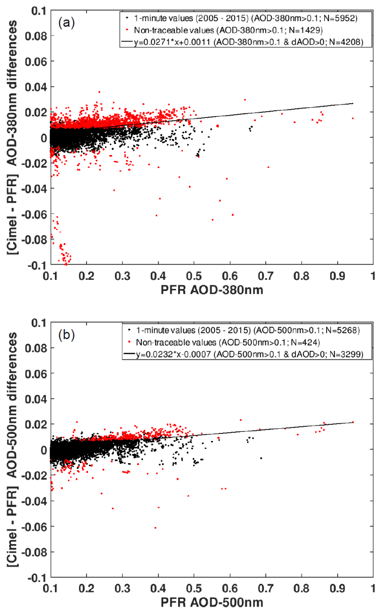
Figure 7. Actual AOD differences between AERONET-Cimel V2 and GAW-PFR vs AOD_{PFR} at (a) 380 nm (b) and 500 nm for the period 2005-2015. The fitting line has been calculated with those data points with AOD > 0.1 and Cimel-PFR AOD difference > 0 . The number of data used in the plots are indicated in the legend. The percentage of non-traceable AOD data with these conditions is \sim 24\% for 380 nm, and \sim 8\% for 500 nm. Note that some traceable (black) points show larger AOD differences than non-traceable (red) points because of the air mass dependence of the WMO traceability criterion.
