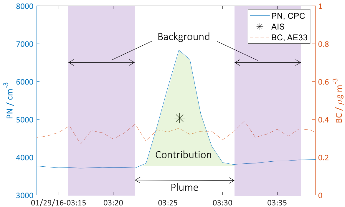
5 Figure 4. Illustration of method of calculating aerosol contribution of individual ship plumes. Particle number concentration measured by a CPC (solid blue) and black carbon measured by an Aethalometer (AE33, dashed orange) during ca 25 minutes of ambient sampling, and calculated time of arrival of the aerosol plume based on AIS and wind data (star). Plume duration is estimated by observation and background concentrations are based on six plus six minutes of adjacent data. The average of the background is subtracted from the plume concentrations to obtain only ship emission contribution.
