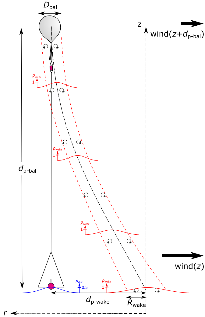
Figure 2. Flow within the LITOS payload chain. d_{\text{p-bal}} : distance between the payload and the centre of the balloon. d_{\text{p-wake}} : distance between the centre of the balloon's wake and the payload. Red lines: distribution of the probability for being in the wake (dashed red line showing the FWHM). Blue line: probability distribution for the payload-wake distance d_{\text{p-wake}} . Sketch is not to scale, the radiosonde below the LITOS gondola is omitted for clarity.
