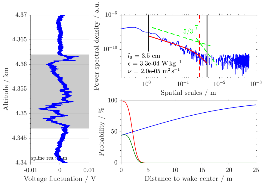
Figure 3. Example for turbulence caused by the balloon’s wake from a LITOS launch on 29 Jan 2016. Left: Raw data from the CTA, grey shaded area influenced by wake. Top right: Turbulence retrieval fit as in Figure 1 from the data shown in the shaded area. Bottom right: Result from the wake prediction algorithm for the same altitude. Blue: Probability distribution of the payload-wake distance d_{p-wake} to be in the range of [0, d] after Equation 12. Red: Radial probability distribution of the wake after Equation 13. Green: Combined probability for wake encounter P_{wake} according to Equation 16.
