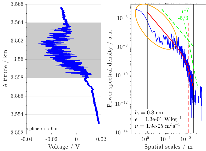
Figure 9. Wake of a rope holding the gondola. Left: Raw data from the CTA. Right: Turbulence retrieval fit as in Figure 1 from the data shown in the left panel. The orange ellipse denotes a region of reduced power spectral densities compared to the Heisenberg model (Eq. 1). This points to turbulence in the wake of a small object in the vicinity of the sensor.
