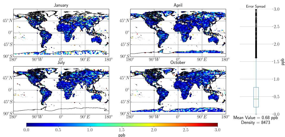
Figure 4. Global Global spread of total error based on the RemoTeC synthetic data ensemble, with ^{13}\text{CH}_4 as the target for retrievals. The four main seasons in the synthetic database are represented in this figure by one day in the months of January, April, July and October. The far right panel in the figure outlines the spread of error values over the entire dataset, with the mean value, and the total number of measurements indicated at the bottom, the circles are outlier values.
