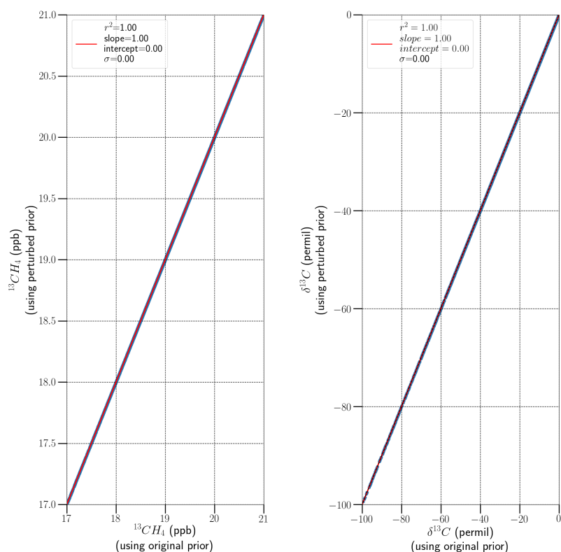
Figure 5. Comparison of retrieved ^{13}\text{CH}_4 (left panel) and \delta^{13}\text{C} (right panel) before and after a priori modification by applying a 2% bias on the methane a priori . The red line is a line of best fit, and the statistical characteristics (coefficient of correlation, gradient, intercept and standard deviation of the difference) are indicated in the legend.
