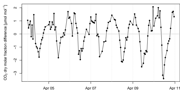
Figure 11. Difference in dry mole fractions of CO 2 between the updraft and downdraft reservoirs of the true eddy accumulation device. The '30-min raw' time series shown is the result of subtracting the mole fraction in the downdraft reservoir from the mole fraction in the updraft reservoir (Fig. 10). A positive CO 2 mole fraction difference indicates a CO 2 flux away from the surface (respiration) and a negative CO 2 mole fraction difference indicates a CO 2 flux towards the surface (assimilation).
