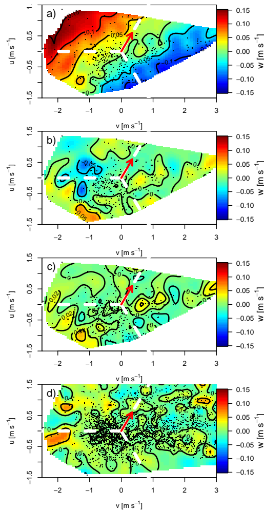
Figure 16. 30-min mean vertical wind velocity w as a function of horizontal wind velocities u and v before and after planar fit coordinate rotation for two different planar fit procedures and two periods. Wind velocities were obtained by the Gill-R3 sonic anemometer which was used for true eddy accumulation. a) Unrotated vertical wind velocity; b) Rotated vertical wind velocity from real-time 1-day moving window planar fit rotation performed by TEA system; c) Rotated vertical wind velocity with single planar fit rotation period performed in post-processing; d) Same as c) but for longer period, i.e. from 1 April to 31 May, 2015. The first three Subfigures a) to c) show data from the experimental period of the current study from 4 April to 11 April, 2015. Black dots indicate location of individual 30-min mean vertical wind velocity readings in the u - v velocity space. Red arrows indicate the direction to North. Dashed lines, in white, indicate the azimuth of the vertical stanchions of the sonic head structure relative to the center of the sonic coordinate system.
