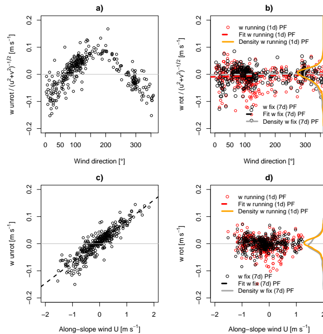
Figure 15. 30-min means of vertical wind velocity, w , before (a, c) and after (b, d) coordinate rotation as a function of wind direction (a, b), and as a function of along-slope wind, U , (c, d). The vertical wind velocity w in a) and b) was normalized by horizontal wind velocity. Subfigures b) and d) both differentiate between two approaches to the planar-fit coordinate rotation: the real-time planar fit applied in the TEA measurements deploying a moving window of one day (“running PF”, in red and orange), and a single planar fit covering the full measurement period (seven days long) obtained in post-processing, (“fix PF”, in black and gray).
