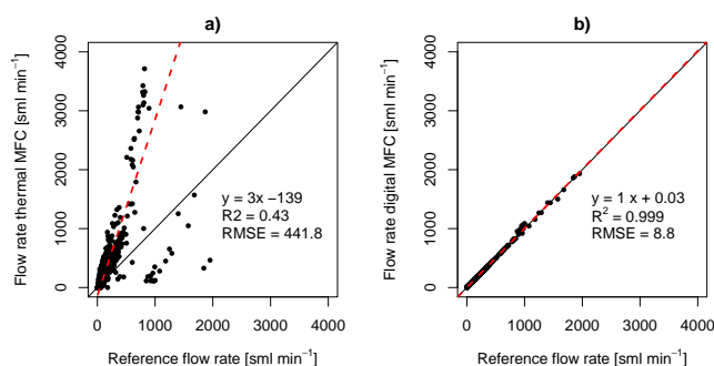
Figure 9. Regression of (a) the thermal mass flow controller flow rate versus the reference flow rate, and (b) the digital mass flow controller flow rate with errors versus the reference flow rate. The reference flow rate was varied at a frequency of 10 Hz proportional to measured vertical wind velocity data. 1:1 line (black solid line), linear model fit (red dashed line). Regression statistics: linear model equation; coefficient of determination, R^2 ; and root mean square error, RMSE.
