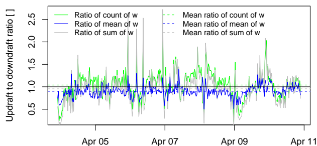
Figure 17. Ratio of statistical measures of vertical wind velocity of updrafts and downdrafts per 30-min flux integration interval. The statistical measures are the ratio of the count, the mean, and the sum of vertical wind velocity records during updrafts and downdrafts, respectively (solid lines). The dashed lines indicate the temporal mean of above statistics over the period displayed.
