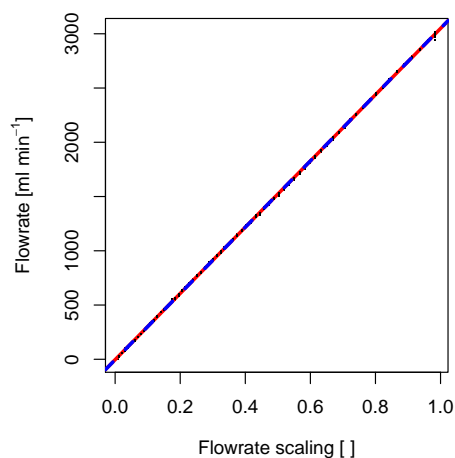
Figure 7. Linearity of two digital mass flow controllers verified by a conventional thermal mass flow controller for a series of 100 constant flow rate levels in the range of 0 to 3000 \text{sml min}^{-1} . The thermal mass flow controller reading is shown on the y-axis versus the set point of the digital mass flow controllers on the x-axis (black dots). The set point range on the x-axis from 0 to 1.0 is linearly related to a flow rate range of 0 to 3000 \text{sml min}^{-1} . Observed linearity errors of the digital mass flow controllers shown here are below 0.3% of the reading. Linear model fit of the digital mass flow controller of the “updraft channel” of the TEA system (red dashed line), and of the “downdraft channel” (blue dashed line), respectively.
