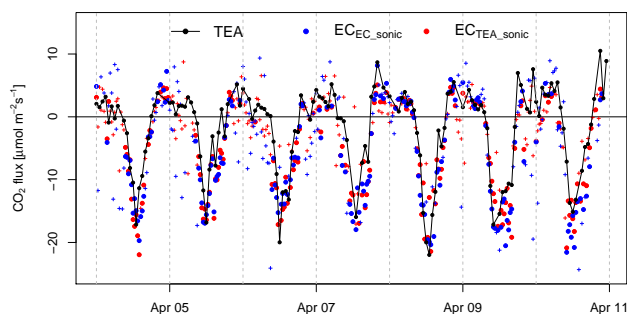
Figure 13. Comparison of CO 2 fluxes measured by true eddy accumulation (TEA) and eddy covariance (EC). Flux integration interval for both methods is 30 min. TEA fluxes were obtained every 60 min and EC fluxes every 30 min. The EC fluxes are quality flag filtered, accepting flags \leq 1 on a scale of 0 to 2 (Foken et al., 2004). The two alternative EC flux calculations shown, in blue and red, respectively, are from two separate Gill-R3 sonic anemometers using CO 2 density data from the same LI-7500 gas analyzer. The symbols indicate if EC flux estimates from the two sonic anemometers were within 50% from each other (full circles) or not (crosses).
