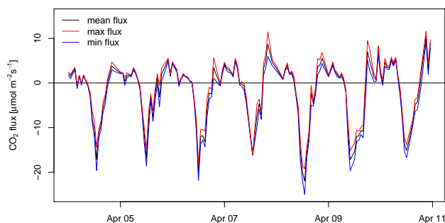
Figure 21. Range of CO 2 trace gas flux estimates observed by the true eddy accumulation method, accounting for the range of possible flux estimates from four replicated measurements of the dry molar fraction difference between accumulated updrafts and downdrafts per 30-min flux integration interval.
