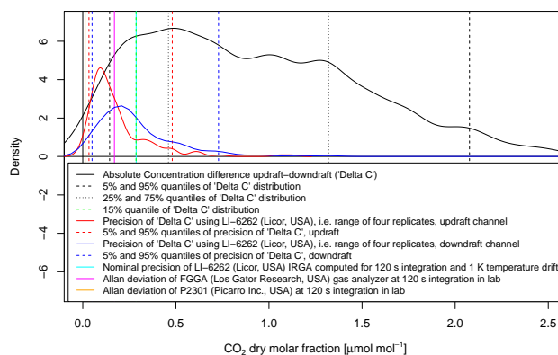
Figure 19. Density distributions and selected probabilities of the trace gas concentration difference signal and of the measurement uncertainties, and gas analyzer precision. The signal is the difference in molar fraction between accumulated updrafts and downdrafts (black line). The uncertainty of the measurements is expressed as the range of four replicated samples of the updraft and downdraft concentration, in red and blue, respectively. Vertical dashed lines indicate various probabilities of above distributions. Vertical solid lines indicate the nominal precision of the LI-6262 (LI-COR, USA) infrared gas analyzer used in this study, calculated for an integration time of 120 s (cyan). Precision of two types of laser spectrometers are also shown for reference: Allan-deviation of FGGA (Los Gatos Research, USA), in magenta, and G2301 (Picarro, USA), in orange, both determined in the laboratory.
