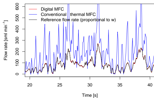
Figure 8. Mass flow rate readings of a conventional thermal mass flow controller (Voegtlin ready-smart series), in blue, measuring a dynamically changing reference flow (black). The magnitude of the reference flow rate, which is proportional to the magnitude of recorded vertical wind velocity data, varied at a frequency of 10 Hz. The reference flow (black) was generated using the new digital mass flow controller. The uncertainty range of the digital mass flow controller (red) is small. On the contrary, the mass flow reading of the conventional thermal mass flow controller deviates significantly from the reference as the conventional mass flow controller is unable to follow the highly dynamic reference signal.
