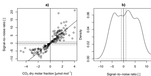
Figure 20. (a) Signal-to-noise ratio ( SNR ) of the trace gas dry molar fraction difference measurements as a function of the this difference, the latter being proportional to the trace gas flux. The solid line is a linear model fit using ordinary-least-squares regression. (b) Density distribution of the signal-to-noise ratio. Dashed lines in (a) and (b) indicate a signal-to-noise ratio of \pm 1 , corresponding to probabilities of 37.7% and 49.5%, respectively. Consequently, in 88% of the cases the signal-to-noise ratio is higher than one, leaving 12% of the cases unresolved. The display in (a) excludes one extreme value at SNR = -66.7 .
