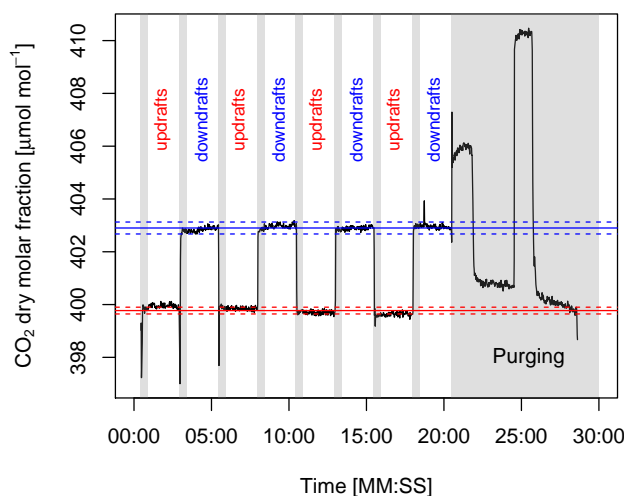
Figure 5. CO 2 dry molar fraction measured as a sequence alternating between updraft and downdraft reservoirs. First the updraft reservoir was measured for 150 s, then the downdraft reservoir for 150 s, discarding the initial 30 s of measurements from each block. This sequence was repeated four times. During the remaining 10 min of the 30 min period any remaining air in the reservoirs was purged and not used for analysis (gray shaded area). The mean of the despiked updraft and downdraft dry molar fractions are indicated by a red and blue solid line, respectively. The dashed lines indicate the mean \pm 1 standard deviation. The start date of the time series is 2015-04-10 13:00:00 UTC.
