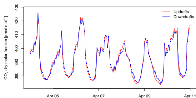
Figure 10. Dry molar fraction of CO 2 in the updraft and downdraft reservoirs of the true eddy accumulation device, in red and blue respectively. The difference in molar fraction is a result of the vertical CO 2 flux.
