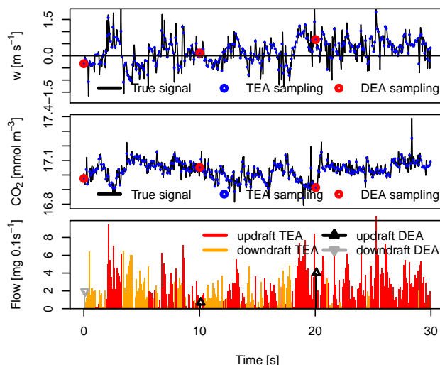
Figure 1. True eddy accumulation and disjunct eddy accumulation sampling scheme. Vertical wind, w , (top panel), scalar density, \text{CO}_2 , (center panel) and vertical wind proportional mass flow rate (bottom panel). Black solid lines indicate the continuous true atmospheric signal. Sampling resolution of TEA and DEA are 10 Hz and 10 s, respectively. Note that active sampling time for DEA is only 1% of the sampling time for TEA.
