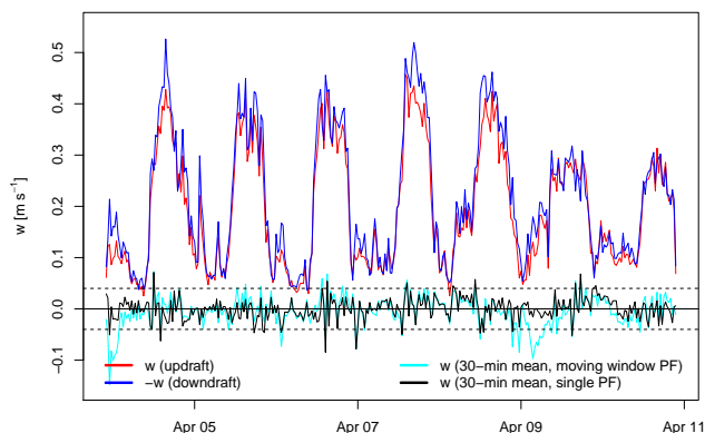
Figure 12. Vertical wind velocity of updrafts and downdrafts, in red and blue, respectively, averaged to 30-min resolution and shown as absolute values. Vertical velocity is subject to a 1 day running window real-time planar fit coordinate rotation as obtained from the TEA system. Mean vertical wind velocity at 30-min resolution after running window real-time planar fit coordinate rotation, in blue, and after a post-processing planar fit coordinate rotation with the fit period corresponding to the full period shown, in black.
