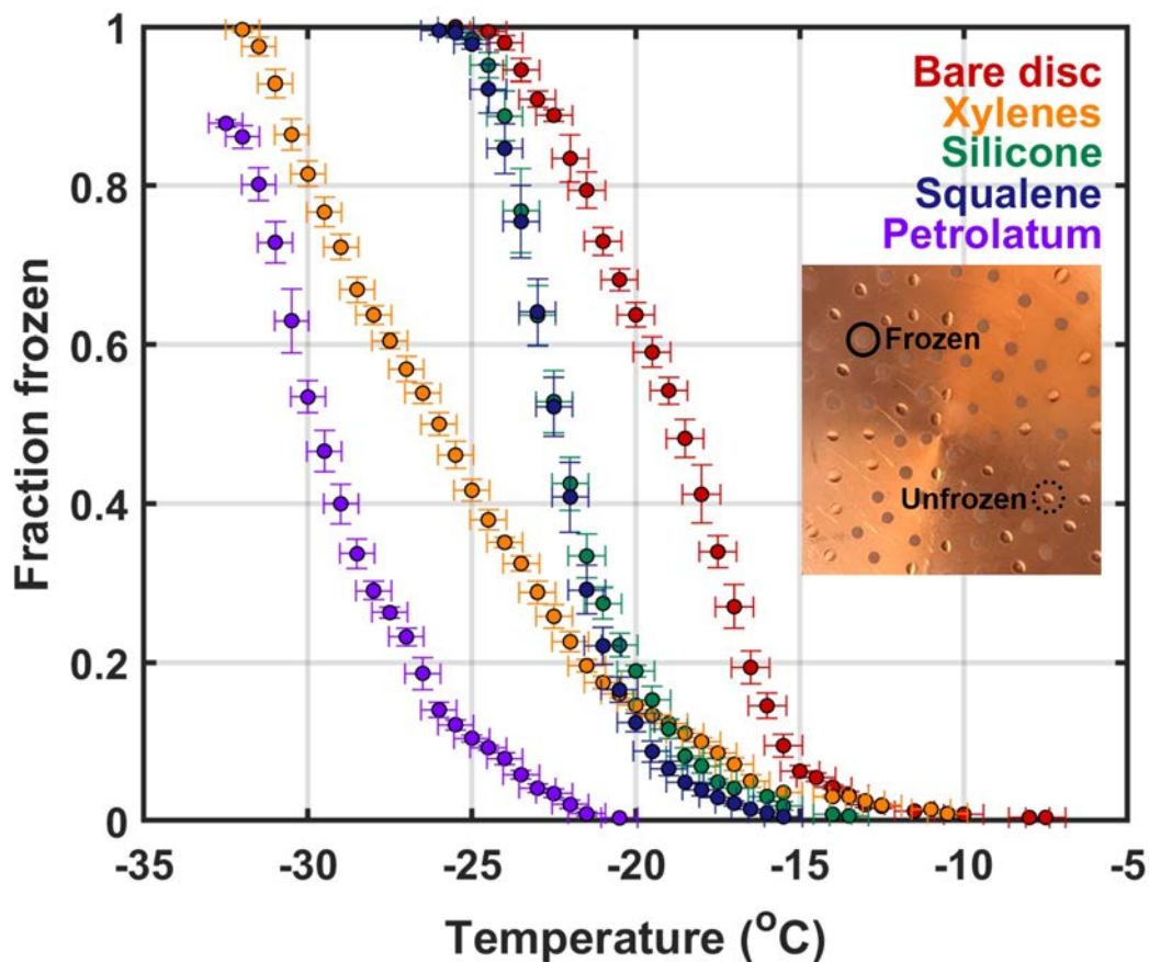
5 Figure 4: Freezing spectra for the control experiments conducted to characterize the DFCP system. Results included here are tests evaluating the most proficient hydrophobic coating with blank UPW drops. Error bars for the y and x axes correspond to standard deviation per 0.5 °C bin and temperature probe/plate versus drop variability standard deviation, respectively. Spectra that do not reach a frozen fraction of 1 indicates not all drops froze at the lower limit of the DFCP. The inset shows an example of the appearance of frozen versus unfrozen 2.5-µL drops on the copper disc.
