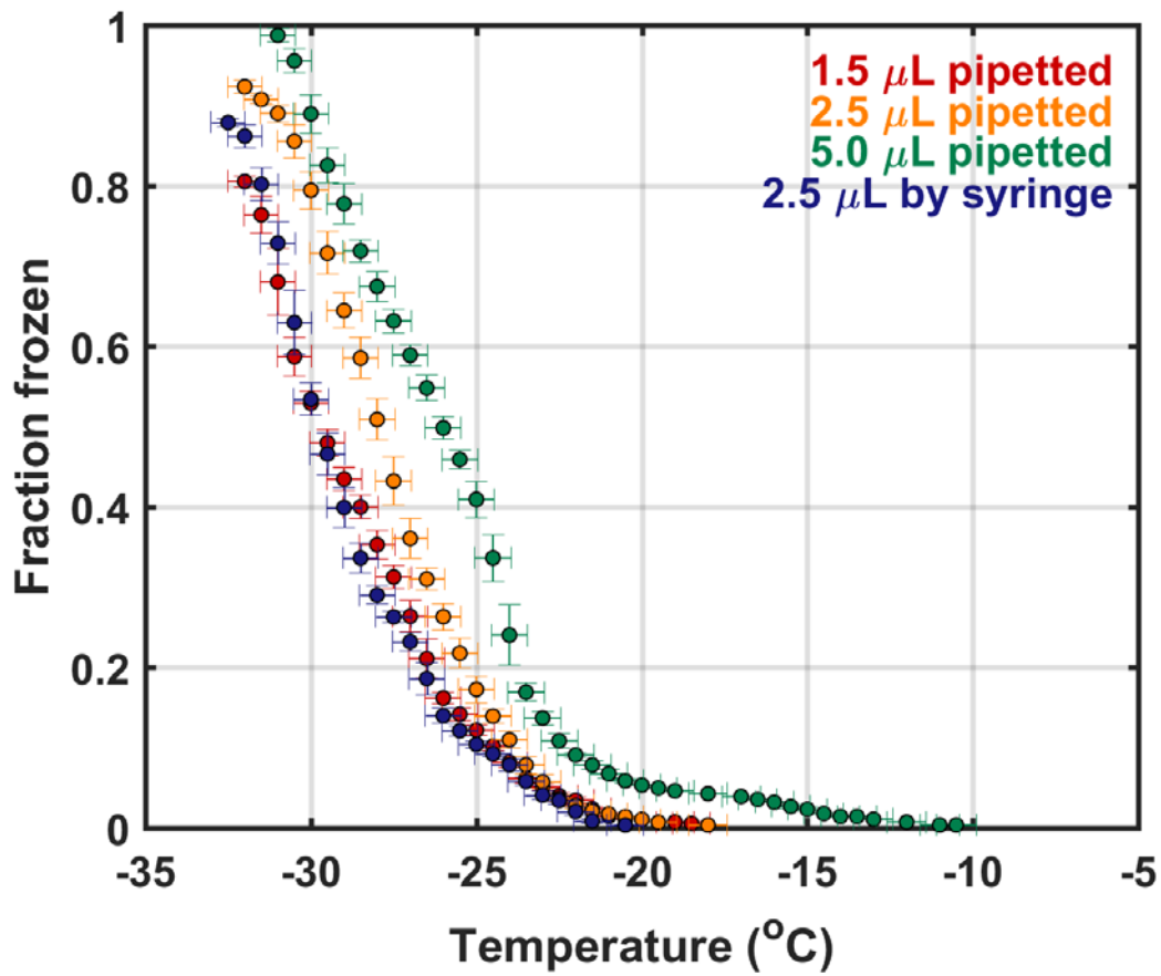
5 Figure 5: Freezing spectra for the control experiments conducted to characterize the drop size chosen for DFCP analysis. Results included here are tests evaluating pipetted versus hand syringe-aliquoted drops and at different volumes. Error bars for the y and x axes correspond to standard deviation per 0.5 °C bin and temperature probe/plate versus drop variability standard deviation, respectively. Spectra that do not reach a frozen fraction of 1 indicates not all drops froze at the lower limit of the DFCP.
