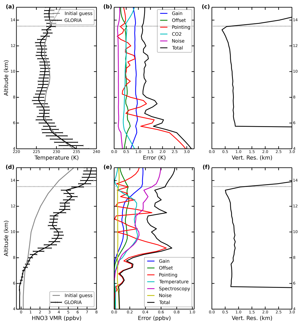
Figure 4. Illustration of the error budget of the temperature and HNO 3 retrieval of Flight 19 on 13 March 2016 for a selected profile at 10:37:06 UTC. First column: retrieved vertical profile of temperature (first row) and HNO 3 (second row) with total estimated error (black) and initial guess profile (grey). The retrieved profile has 14.9 and 12.5 degrees of freedom for temperature and HNO 3 , respectively. Second column: Different total error contributions and estimated total error. Last column: Vertical resolution of this retrieval result. The dotted line represents the flight altitude of the aircraft.
