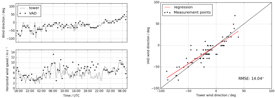
Figure 5. Comparison of lidar #3 VAD scans with sonic anemometer measurements at 80 m on tower 20/tse04 from 17th to 19th of May. On the left a comparison of the time series of wind direction and wind speed, and on the right a regression plot of wind directions.
