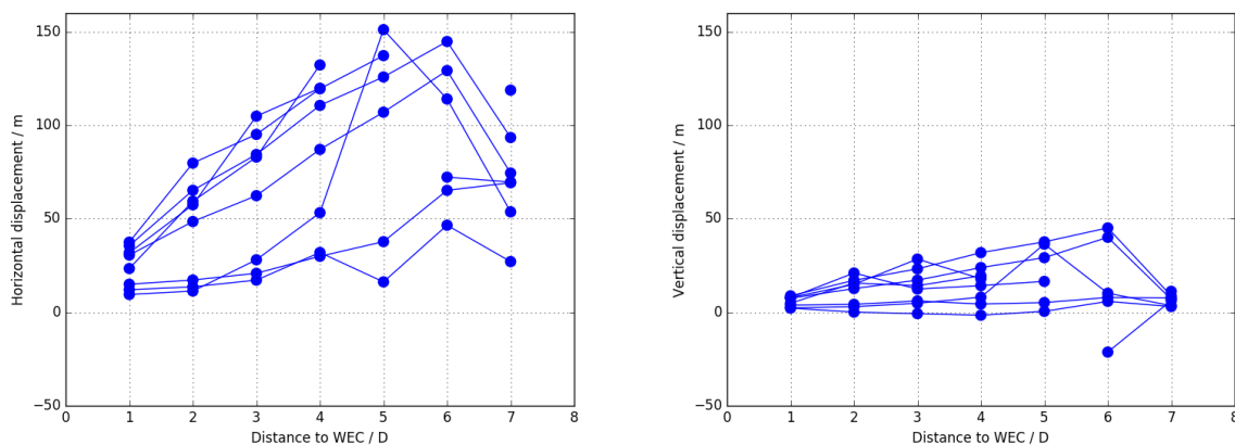
Figure 10. Averaged misalignment of the determined wake center to the beam crossing measurement point.
