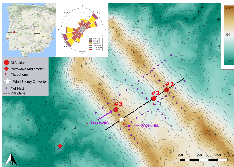
Figure 1. Map of the Perdigo site, including DLR instrumentation and meteorological mast locations. It also shows a wind rose for the sonic anemometer at 80 m on tower 20/tse04 for the IOP period. The dashed black line indicates the typical RHI scanning plane.
