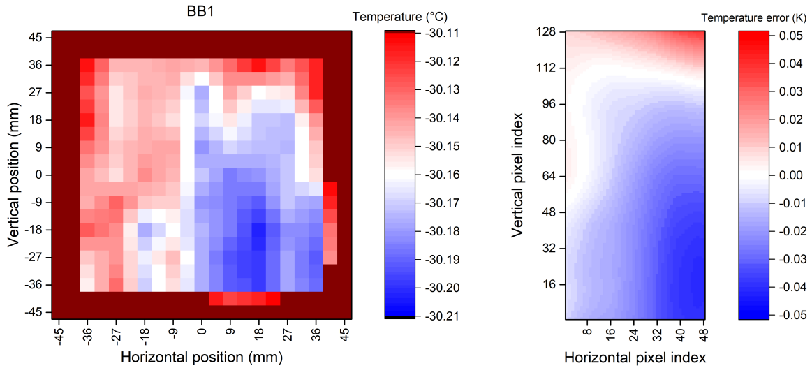
Figure 8. Measured surface radiance temperatures at -30.15^{\circ}\text{C} (243 K) for BB1 (left) and estimated resulting temperature error for each of the 48 x 128 detector pixels (right)
