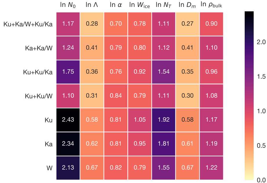
Figure 5. The average posterior retrieval errors of the logarithms of microphysical variables with different combinations of radar frequencies. The data from the December 4, 2015, case (Sect. 5.2) is are used in this figure.
