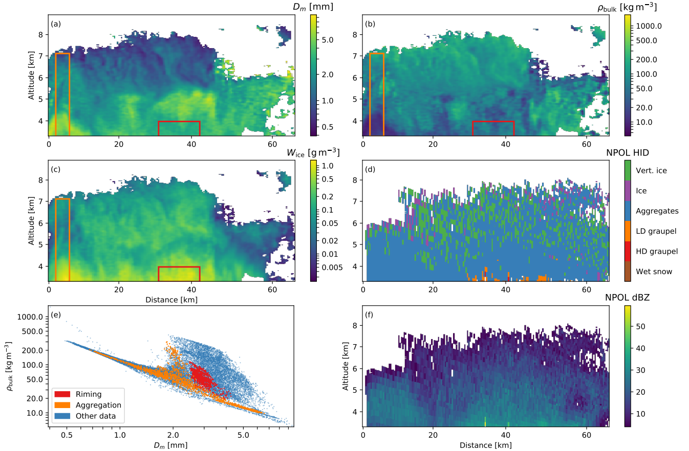
Figure 2. Data from the December 3, 2015 case, described in Sect. 5.1. (a) The mass-weighted mean diameter D_m (Eq. 14). (b) The bulk density \rho_{\text{bulk}} (Eq. 16). (c) The ice water content (Eq. 12). (d) The NPOL hydrometeor identification. (e) A scatter plot of D_m and \rho_{\text{bulk}} from panels a and b, with the red and orange points identifying the data inside the boxes of corresponding colors shown on those panels. (f) The radar reflectivity observed by NPOL. The location of NPOL on the flight track is marked on panels a–d and f.
