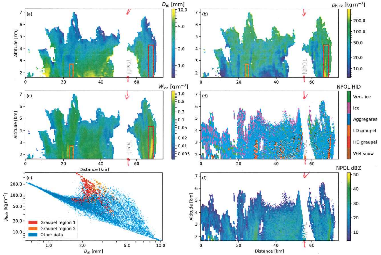
Figure 3. As Fig. 2, except for the December 4, 2015 case described in Sect. 5.2
