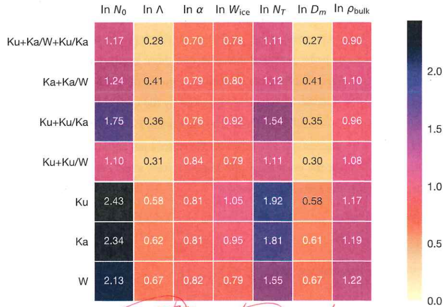
Figure 5. The average posterior retrieval errors of the logarithms of microphysical variables with different combinations of radar frequencies. The data from the December 4, 2015, case (Sect. 5.2) is used in this figure.
