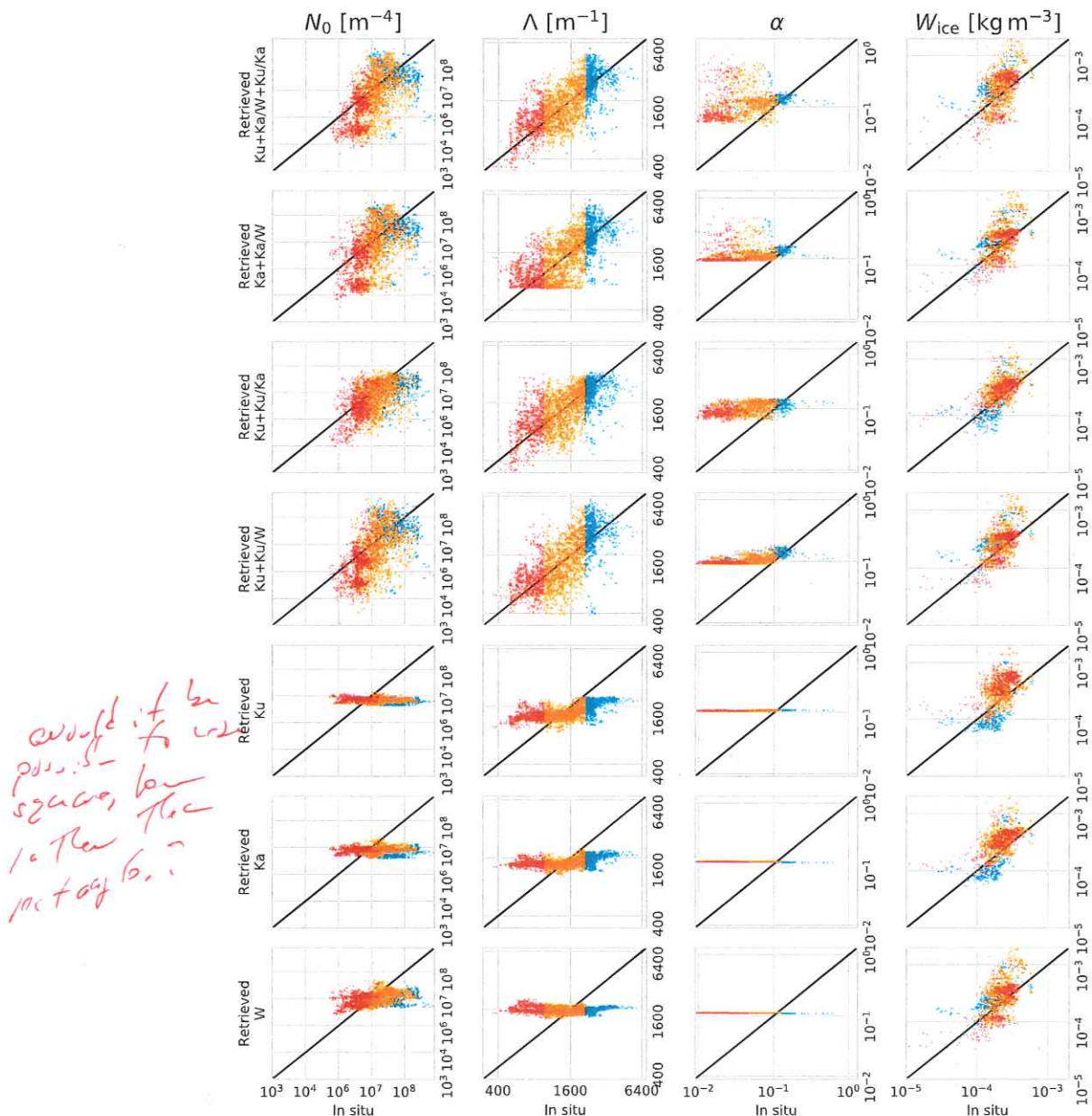
Figure 4. Scatter plots of in situ measured (horizontal axis) and retrieved (vertical axis) microphysical values from the collocated Citation/APR-3 dataset. The columns correspond to different microphysical parameters: from left to right, the intercept parameter N_0 ; the slope parameter \Lambda ; the mass-dimensional prefactor \alpha ; and the ice water content W_{ice} . The rows correspond to different combinations of radar frequencies and DWRs used to run the retrieval, as shown to the left of each row. The color denotes the size of the snowflakes: Blue dots correspond to small particles (largest 25% of \Lambda ), orange to medium-sized particles, and red to large particles (smallest 25% of \Lambda ). On each plot, the black line is the 1 : 1 line. Note the logarithmic scales on the axes.
