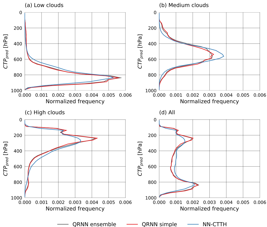
Figure 9. Error-distributions Distributions of predicted CTP values ( CTP_{pred} ) with respect to CTP from CALIOP for high clouds in panel (c) ( CTP_{ref} ) , medium clouds in panel (b) , low clouds in panel (a) for different cloud types and the complete test set in panel (d) .
