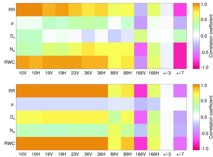
Figure 4. Correlations of T_B at GMI frequencies with the DSD parameters (Eq. 1) as well as rain rate (RR) and RWC, as derived from disdrometer measurements run through a RT model. Convective DSDs (top) and stratiform DSDs (bottom) are shown for extratropical ocean cases.
