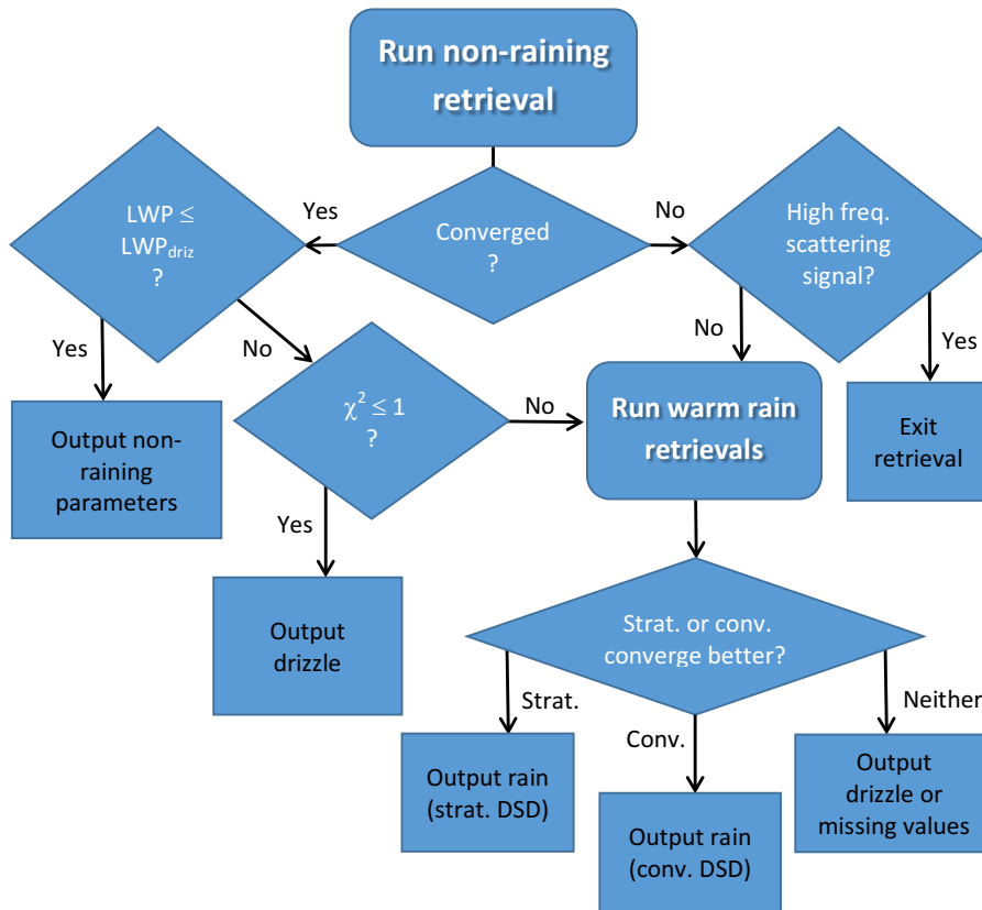
Figure 6. Algorithm flowchart for the IDVAR for warm rain.
