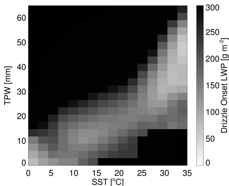
Figure 1. Drizzle onset value of LWP, separated by SST and TPW. Regimes with no data are assigned the maximum value, 300\ \text{g m}^{-2} .
