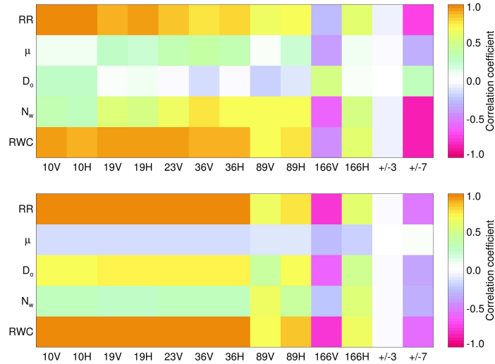
Figure 4. Correlations of T_B at GMI frequencies with the DSD parameters (Eq. 1) as well as rain rate and RWC, as derived from disdrometer measurements run through a RT model. Convective DSDs (top) and stratiform DSDs (bottom) are shown for extratropical ocean cases.
