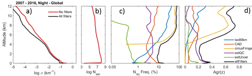
Figure 20. (a) Mean extinction with and without quality filters, (b) number of unfiltered aerosol samples, (c) frequency of aerosol samples rejected, and (d) filter aggressiveness (Eq. (A4B1)) smoothed vertically over 600 m for 2007–2016 at night, all-sky.
