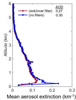
Figure 17. Level 3 \bar{\sigma} with the extinction uncertainty filter (red) and with no filters (blue) over the South America region (Table B4A1) for 2010 at night, all-sky.
