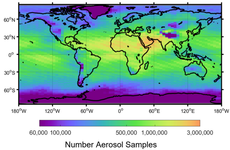
Figure S1. Total number of aerosol samples reported by the level 3 product prior to data filtering quality screening for 2007–2016 at day, all-sky.
