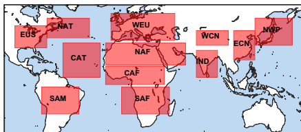
Figure 21. Region definitions, similar to those defined by Yu et al. (2010): EUS = Eastern United States, WEU = Western Europe, IND = India, ECN = Eastern China, NAT = North Atlantic Ocean, CAT = Central Atlantic Ocean, NWP = Northwest Pacific Ocean, NAF = North Africa, WCN = Western China, SAM = South America, CAF = Central Africa, SAF = Southern Africa. Geographic boundaries are specified in Table B4A1.
