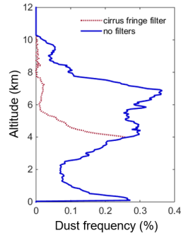
Figure 13. Dust detection frequency ( 100 \times N_{\text{dust}} / N_{\text{all aerosol}} ) with and without the cirrus fringe filter for September – November 2010 at night over the south Pacific Ocean [30° S, 55° S; 80° W, 180° W].
