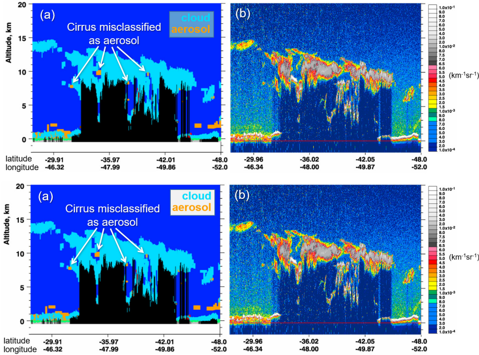
Figure 12. (a) Feature type classification and (b) total attenuated backscatter showing cirrus misclassified as aerosol for the version 3 granule 2011-11-10T03-54-52Z.
