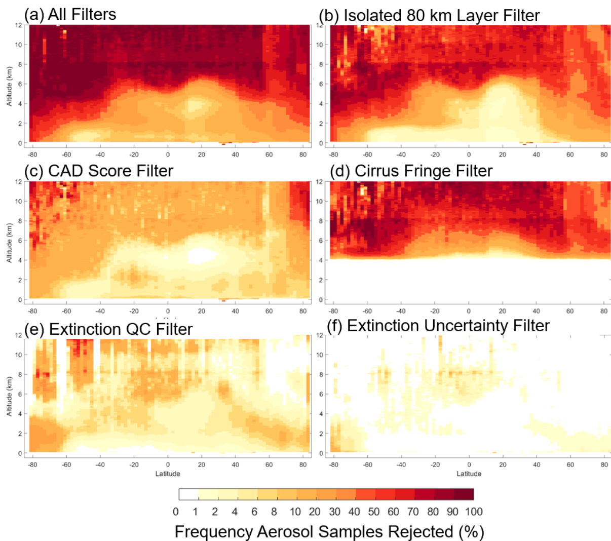
Figure S4. Zonal frequency of aerosol samples rejected by the indicated filter out of all aerosol detected as reported by the level 3 product for 2007–2016 at day, all-sky.
