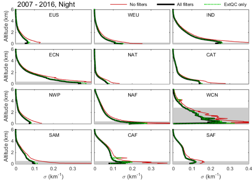
Figure 22. Regional \bar{\sigma} with no filters (red), all filters (black), and the extinction QC filter only (green dashed) for 2007–2016 at night, all-sky. The median surface elevation indicated by the shaded grey region.
