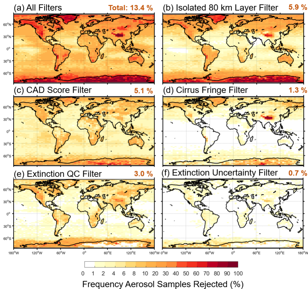
Figure S3. Frequency of aerosol samples rejected by the indicated filter out of all aerosol detected as reported by the level 3 product for 2007–2016 at day, all-sky. Global total rejection frequencies are indicated in the panel titles.
