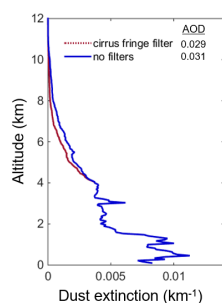
Figure 14. Mean dust extinction with and without cirrus fringe filter for March – May MAM 2010 at night over the Asian dust outflow region [30° N, 60° N; 140° E, 180° E].
