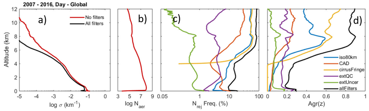
Figure S6. (a) Mean extinction with and without quality filters, (b) number of unfiltered aerosol samples, (c) frequency of aerosol samples rejected, and (d) filter aggressiveness (Eq. (A1B1)) smoothed vertically over 600 meters for 2007–2016 at day, all-sky.
