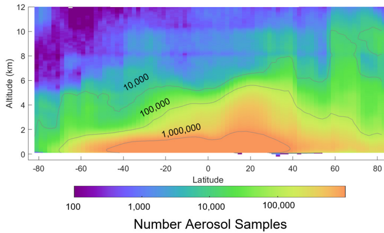
Figure S2. Zonal total number of aerosol samples reported by the level 3 product prior to data filtering quality screening for 2007–2016 at day, all-sky.
