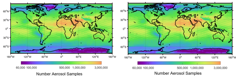
Figure 6. Total number of aerosol samples reported by the level 3 product prior to quality screening for 2007–2016 at night, all-sky.
