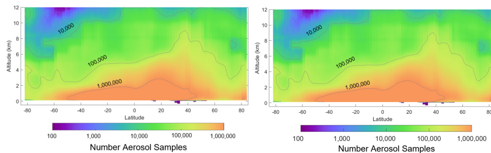
5 Figure 7. Zonal total number of aerosol samples reported by the level 3 product prior to quality screening for 2007–2016 at night, all-sky.
