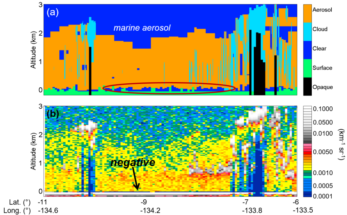
Figure 3. (a) Level 2 feature type classification and (b) level 1B total attenuated backscatter for the granule 2008-08-01T10-17-21ZN passing over the Pacific Ocean. Undetected surface-attached aerosol (circled) and negative attenuated backscatter (arrow) are denoted.
