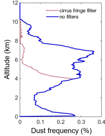
Figure 13. Dust detection frequency ( 100 \times N_{dust} / N_{all\ aerosol} ) with and without the cirrus fringe filter for September – November 2010 at night over the south Pacific Ocean [30° S, 55° S; 80° W, 180° W].
