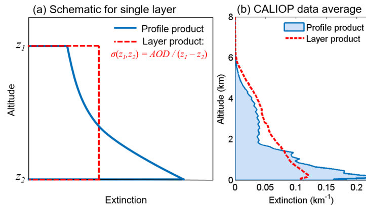
Figure 1. (a) Schematic example of aerosol extinction profile for an individual layer reported by the profile product (blue) and by the layer product (red dashed) where mean aerosol extinction is computed from the layer AOD divided by the geometric depth ( \Delta z ). (b) Seasonal average of CALIOP aerosol extinction computed by the profile product (blue, filled) and by the layer product (red dashed) for June – August 2007 at night over the central Atlantic Ocean region (Table A1).
