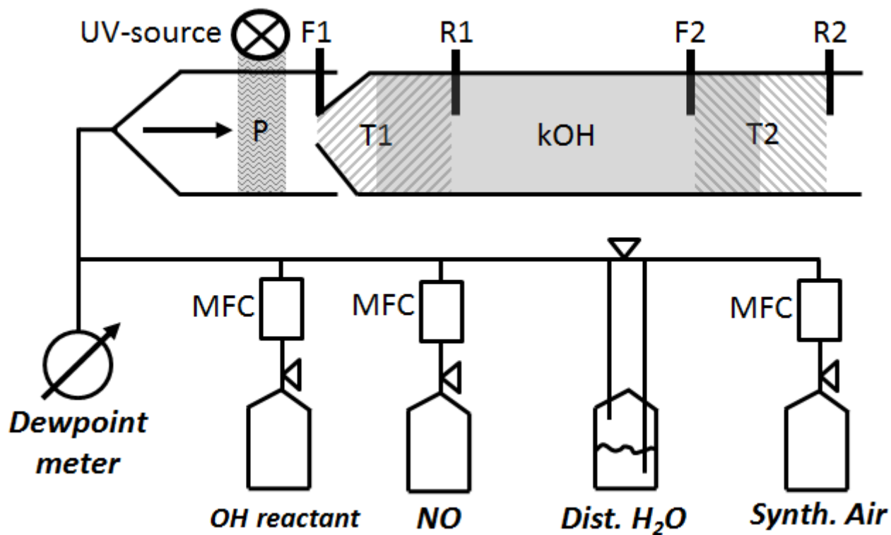
Figure 2: Schematic of CIMS flow tube with two titration zones: P = OH and HO 2 production from H 2 O photolysis. T1 zone (left hatch) = first titration zone (F1 up to R1) with H 2 SO 4 from OH titration by SO 2 injection at F1. T2 zone (right hatch) = second titration zone (F2 up to R2) with H 2 SO 4 from OH titration by SO 2 injection at F2. R1 and R2 = added propane to stop H 2 SO 4 production from recycled OH after the first and second titration zone, respectively. KOH (grey solid) = total OH reactivity using \ln ([OH]_{T1}/[OH]_{T2}) indicating [OH] T1,T2 is reached after front (F1, F2) and before rear (R1, R2) injection.
