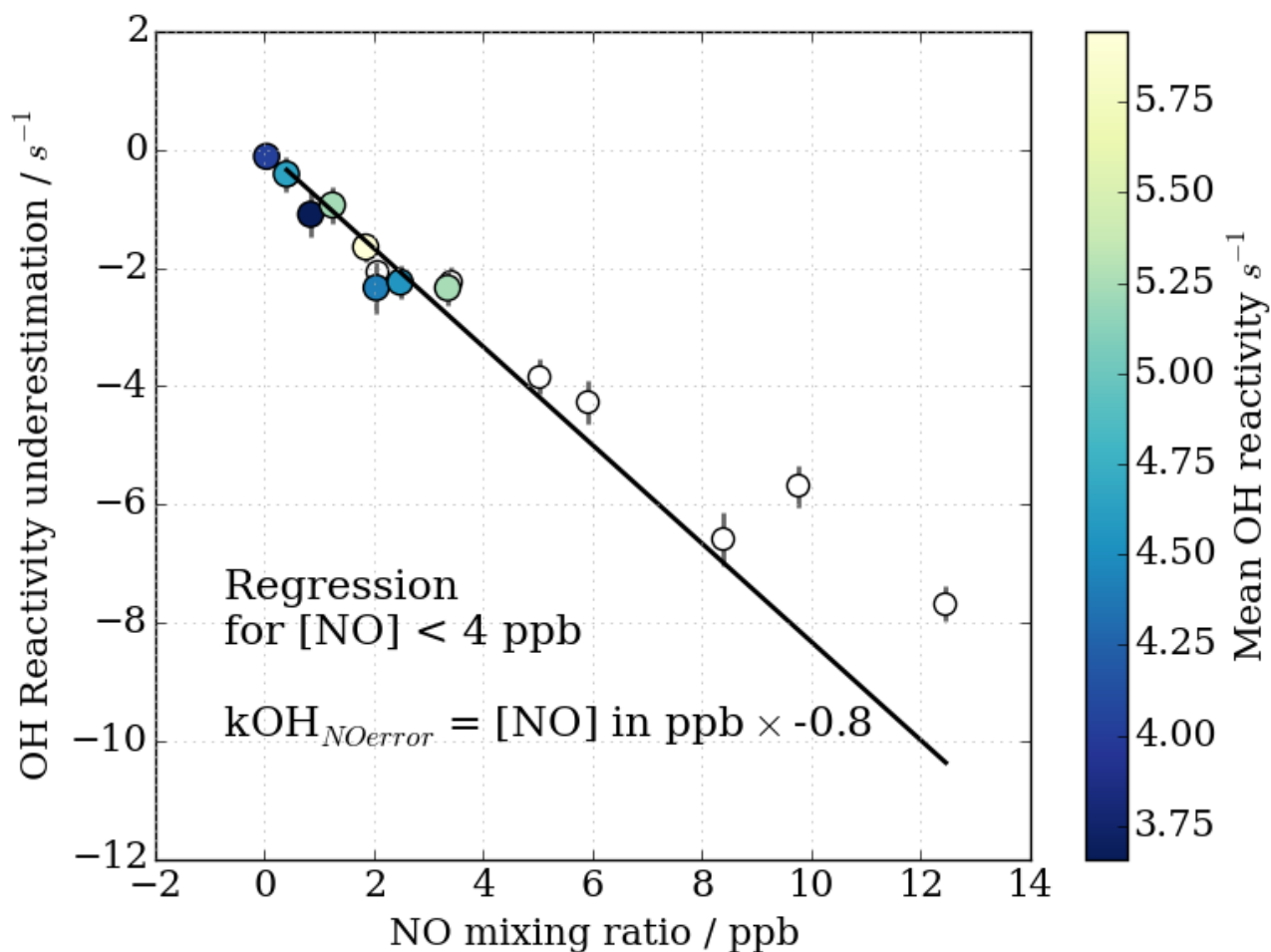
Figure 12: OH reactivity underestimation for MOHp relevant NO mixing ratio and typical OH reactivity (maximum 15 s^{-1} ). Filled circles are data used for linear regression to obtain mean underestimation of OH reactivity for NO up to 4 ppb.
