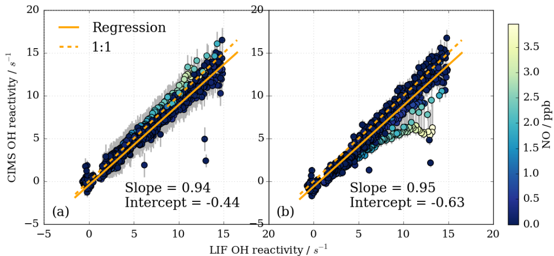
Figure 13: Subset of OH reactivity measurements from instrument comparison (Fuchs et al., 2017) for OH reactivity up to 15 s^{-1} and NO concentrations up to 4 ppb (716 data points). (a) CIMS data treatment includes eight parameter NO correction, (b) CIMS data are not corrected for NO presence, but a positive NO-dependent uncertainty is associated with the measurement (Fig. 12).
