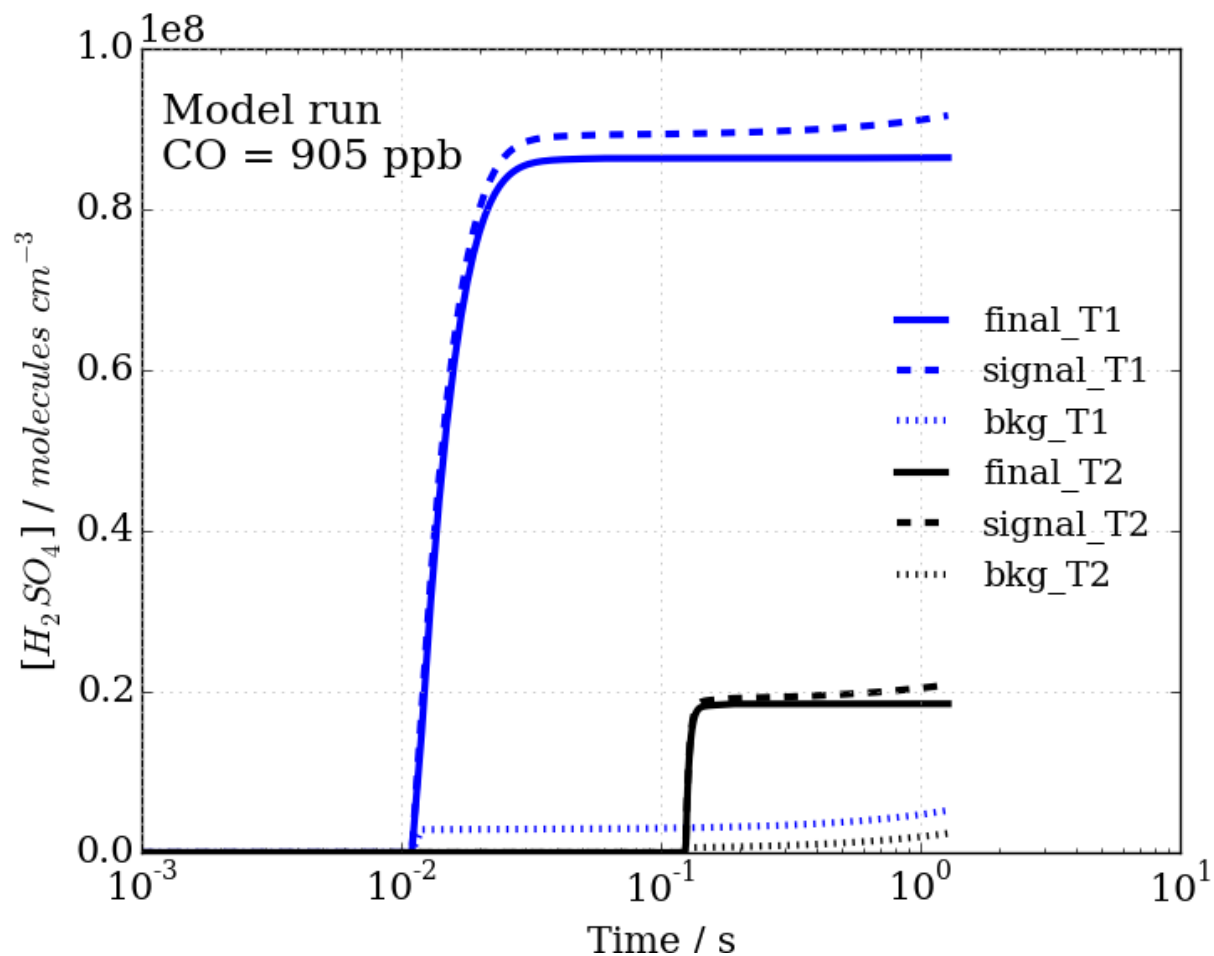
Figure 4: Sulfuric acid concentrations with time, representing progression in sample flow tube from inlet tip to ionisation region, for signal and background modes (dashed and dotted lines respectively), as well as the calculated difference, leading to final [H_2SO_4]_{T1} = [OH]_{T1} and final [H_2SO_4]_{T2} = [OH]_{T2} concentrations (solid lines) in titration zones 1 (T1) and 2 (T2) which are used to calculate OH reactivity.
