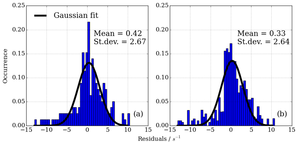
Figure 11: Residuals in CIMS OH reactivity after applying NO correction function. (a) 165 individual points from isoprene, ethene and propane NO correction experiment, (b) 194 individual points from four propane NO correction experiments March 2016 – March 2017. Distribution is normalised according to number of points in each experiment.
