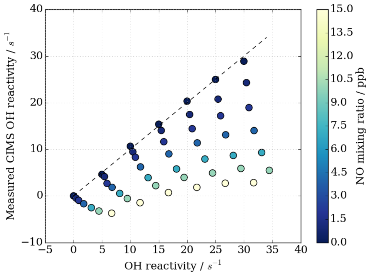
Figure 8: CIMS OH reactivity underestimation as result of NO-HOx recycling interference in external flow tube NO correction experiment. OH reactivity is the average of experiments with OH reactants propane, isoprene, ethene and NO.
