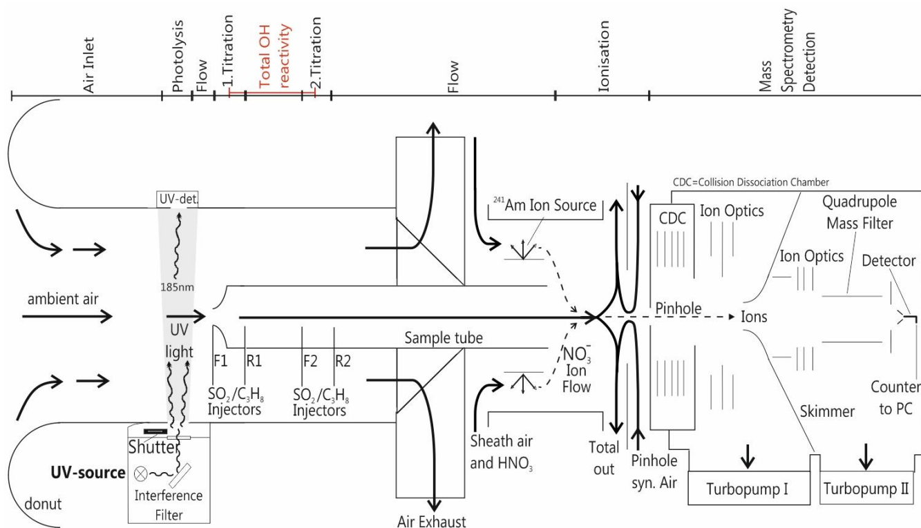
Figure 1: Schematic of CIMS system used for long-term OH, H 2 SO 4 and OH reactivity measurements at the Meteorological Observatory Hohenpeissenberg, Germany. Air flows are indicated by arrows, the measurement zones are described in the upper part of the schematic.
