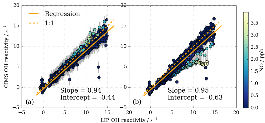
5 Figure 13: Subset of OH reactivity measurements from instrument comparison (Fuchs et al., 2017) for OH reactivity up to 15 \text{ s}^{-1} and NO concentrations up to 4 ppb (716 data points). (a) CIMS data treatment includes eight parameter NO correction, (b) CIMS data are not corrected for NO presence, but a positive NO-dependent uncertainty is associated with the measurement (Fig. 12).
