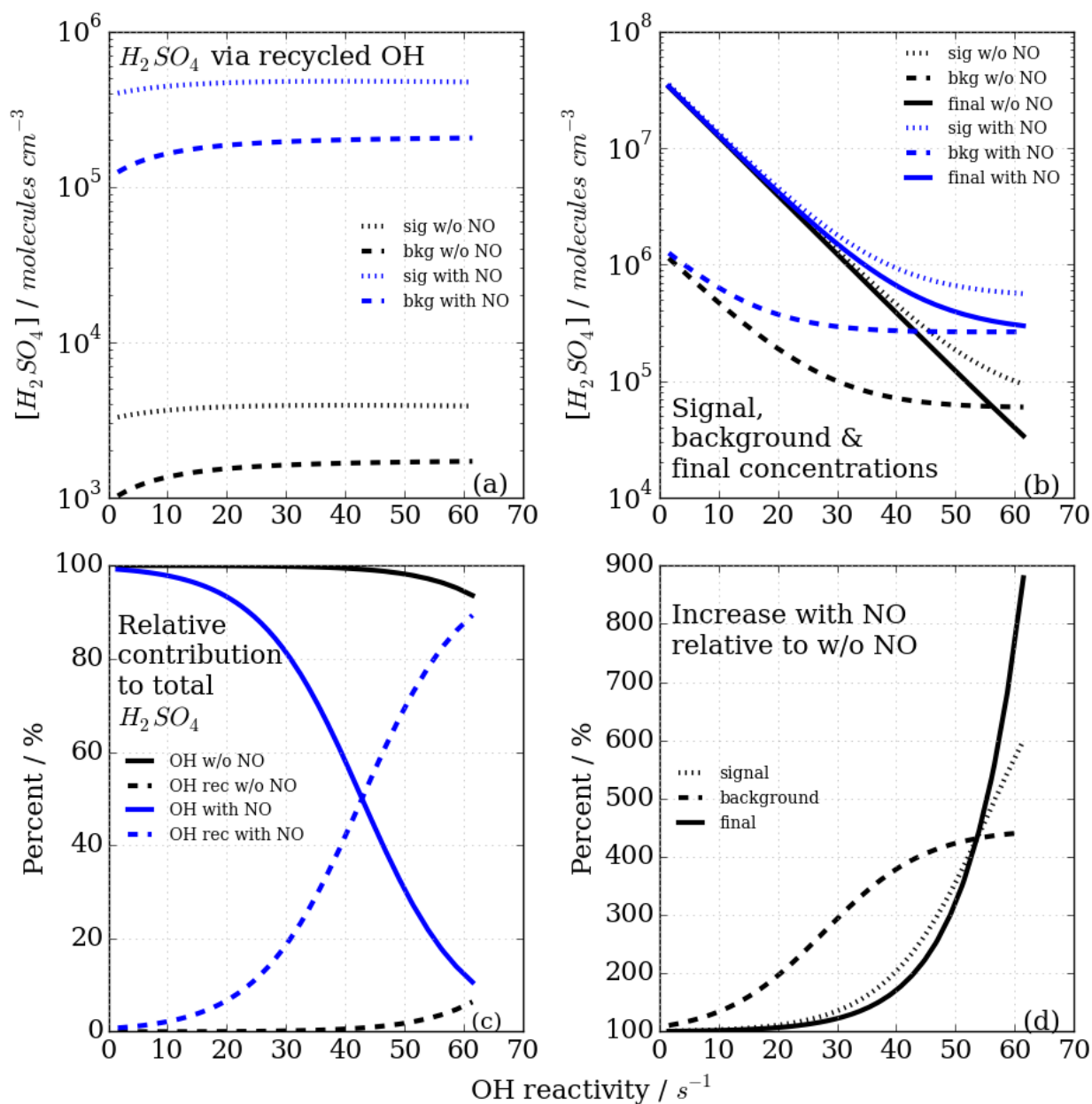
Figure 7: Modelled CIMS H_2SO_4 concentrations and contributions from OH recycling in titration zone 2 with and without NO impurity (140 ppt) present. (a) Absolute H_2SO_4 concentrations from recycled OH only in signal and background measurement mode. (b) Total H_2SO_4 concentrations. (c) Relative contribution from OH_{UV} and OH recycled to the total (and final) H_2SO_4 concentration. (d) Non-linear increases in signal, background and final measurements in case of presence of NO impurity.
