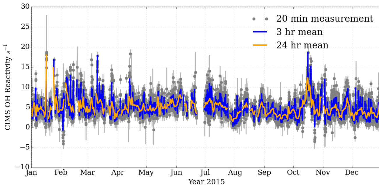
5 Figure 14: OH Reactivity measurements by CIMS at MOHp for the year 2015, with 3 hour and daily means in blue and orange respectively. Filtered for recorded instrumental and laboratory interferences and seven outliers not coinciding with short term CO and NO 2 concentration peaks. 15541 valid measurement points.
