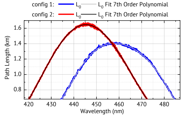
Figure 2. Measured path length \bar{L}_0(\lambda) for a zero air filled cavity for two instrument configurations, both used in this paper. Contributions to the Path-Length by mirror reflectivity, Rayleigh extinction and O_4 absorption are shown for config 1 in the supplement Fig. SF1.
