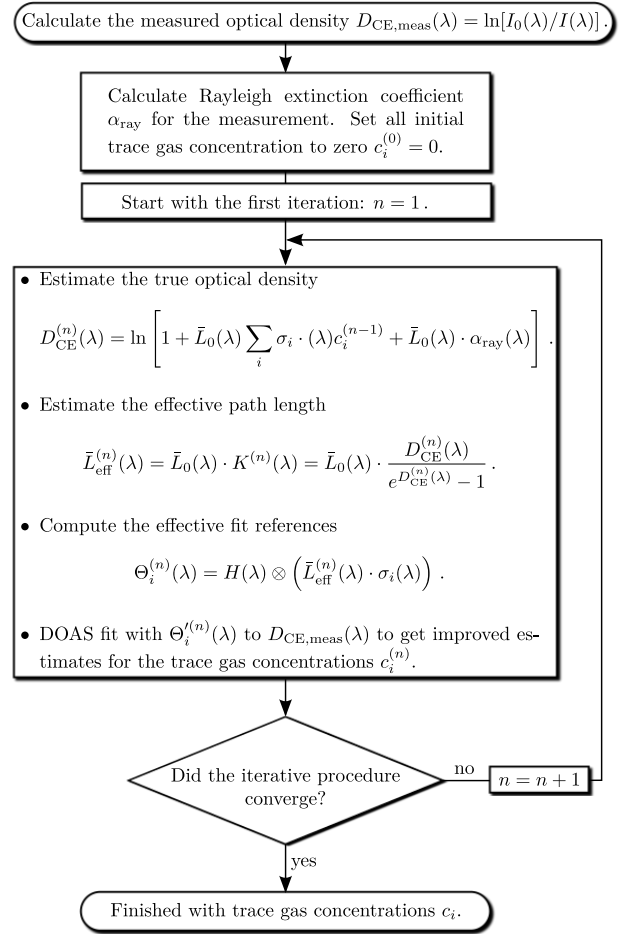
Figure 4. Scheme of the ICAD algorithm
