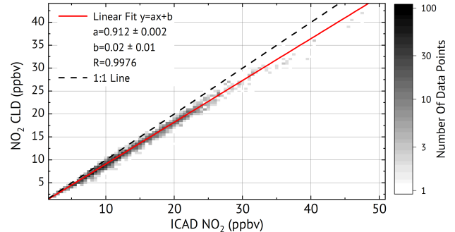
Figure 12. Correlation plot between ICAD \text{NO}_2 and CLD/BLC measurements.
