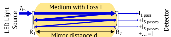
Figure 1. CEAS Principle
