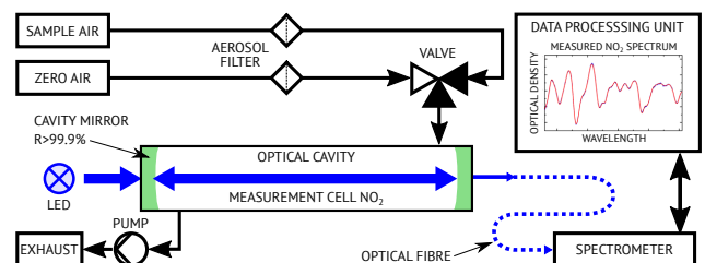
Figure 7. Schematic drawing of the ICAD instrument.
