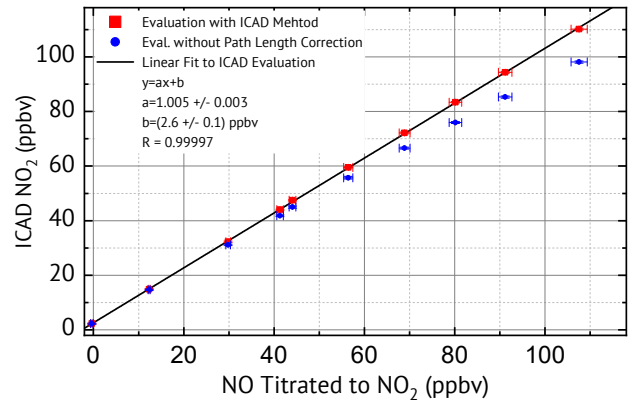
Figure 9. Measurements (spectra recorded with instrument configuration 1) of gas mixtures with different \text{NO}_2 concentration.
