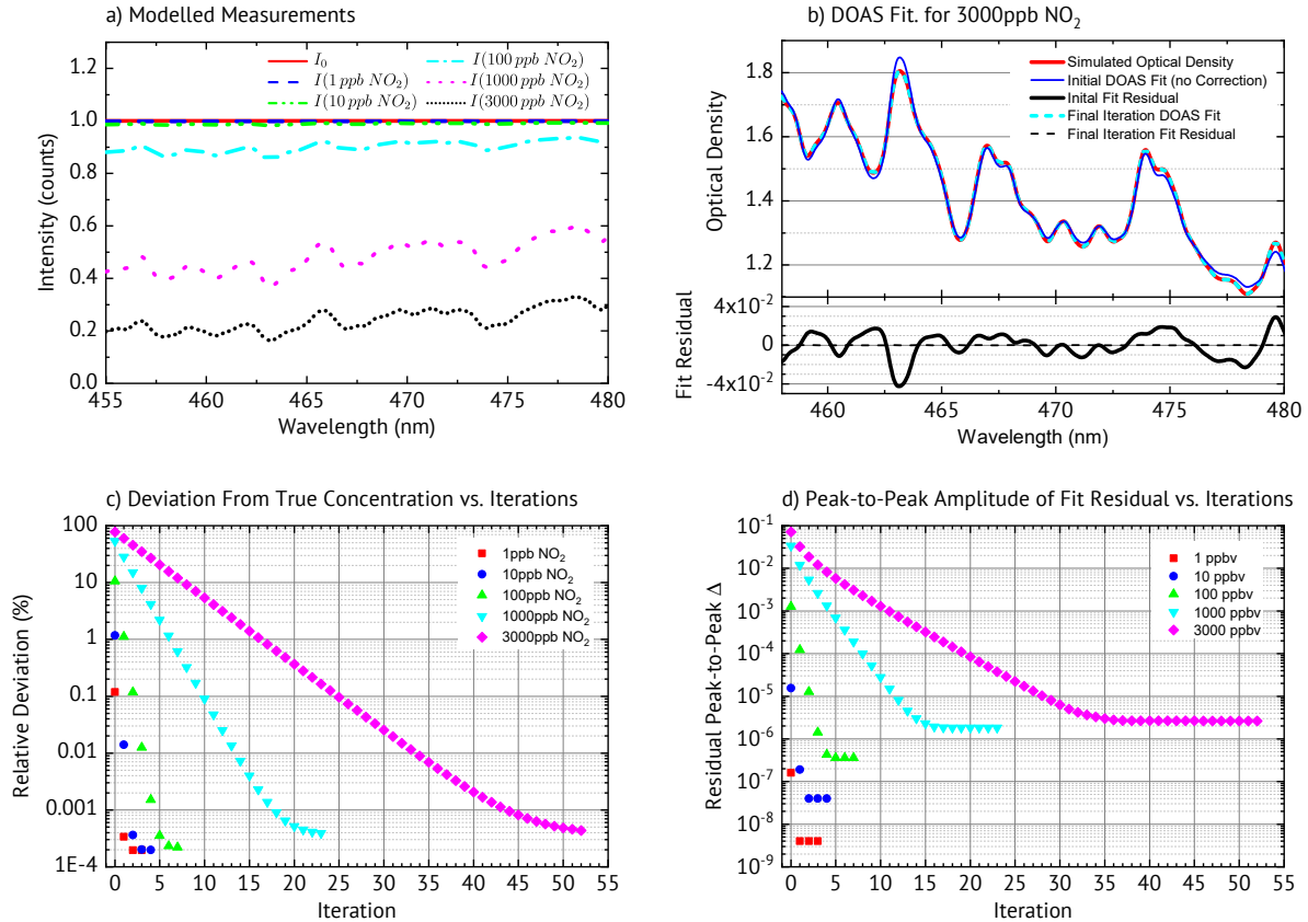
Figure 5. ICAD evaluations of simulated measurements. (a) shows the measured spectra, (modelled without photon shot noise) for different NO 2 mixing ratios (see Sect. 3.1). Panel (b) shows DOAS fits for a NO 2 mixing ratio of 3000 ppbv. It shows the improvement of the DOAS fit from the initial iteration (fitted concentration of 676 ppbv) to the final iteration with optimized fit references (final derived concentration 2999.99 ppbv). In the final iteration the NO 2 absorption bands of the simulated optical density are almost perfectly matched, reducing the fit residual by four orders of magnitude. The convergence of the retrieved NO 2 towards its true value is shown in panel (c) as a function of the ICAD iteration number. Panel (d) shows the improvement of the fit residual during the iterative evaluation. In a real measurement the achievable noise levels are limited by the fundamental photon shot noise and instrumental error sources (see Sect. 4.3).
