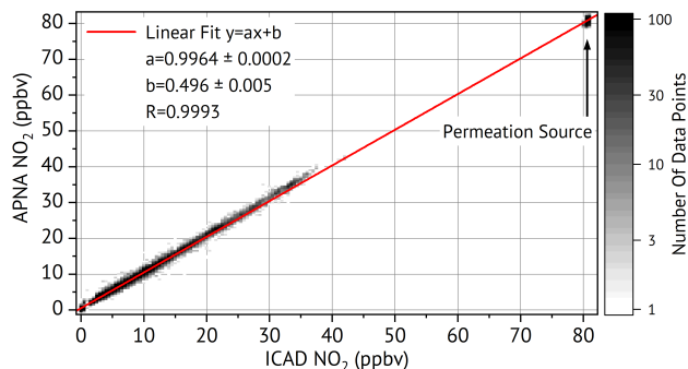
Figure 13. Correlation plot between ICAD \text{NO}_2 A and APNA 370 CLD measurements.
