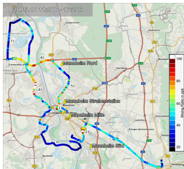
Figure 14. Overview on the car based measurements in the greater Mannheim-Ludwigshafen urban area. The colour of the route segments corresponds to the local \text{NO}_2 mixing ratio. The areas marked on the map are: 1) Mannheim city centre, 2) Mannheim rail road shunting yard, 3) Mannheim suburbs Altrip and Rheingönheim, 4) BASF industrial plant, 5) main road B44, 6) Highway A6, 7) suburb Bobenheim-Roxheim. The yellow pins show the locations of the LUBW, air quality monitoring stations in the measuring area. The map overlay was created with Google Earth. Map information provided by MapQuest, OpenStreetMap, ODbL.
