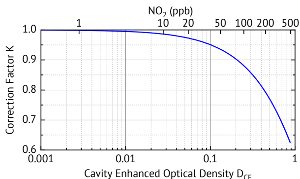
Figure 3. Correction factor K as a function of the Cavity Enhanced Optical Density D_{CE} . Note that the correction factor also is wavelength dependent as the optical density D_{CE}(\lambda) is wavelength dependent.
