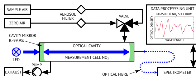
Figure 7. Schematic drawing of the ICAD instrument.
