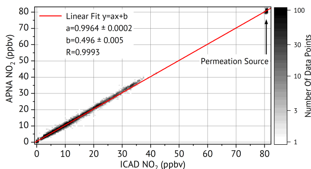
Figure 13. Correlation plot between ICAD NO 2 and APNA 370 CLD measurements.
