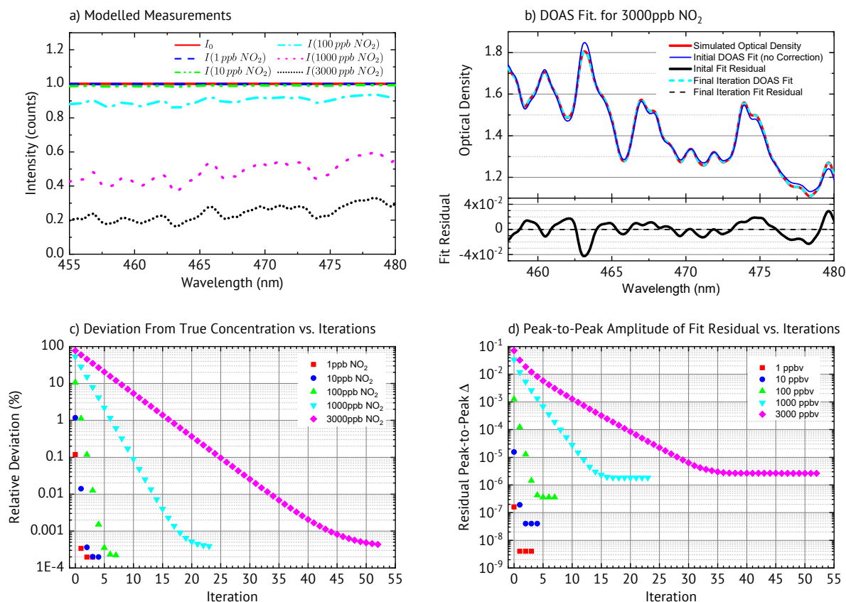
Figure 5. Simulated ICAD evaluations. (a) shows the measured spectra, (modelled without photon shot noise) for different NO 2 mixing ratios (see Sect. 3.1). Panel (b) shows DOAS fits for a NO 2 mixing ratio of 3000 ppbv. It shows the improvement of the DOAS fit from the initial iteration (fitted concentration of 676 ppbv) to the final iteration with optimized fit references (final derived concentration 2999.99 ppbv). In the final iteration the NO 2 absorption bands in the simulated optical density are almost perfectly matched, reducing the fit residual by four orders of magnitude. The convergence of the retrieved NO 2 towards its true value is shown in panel (c) as a function of the ICAD iteration number. Panel (d) shows the improvement of the fit residual during the iterative evaluation.
