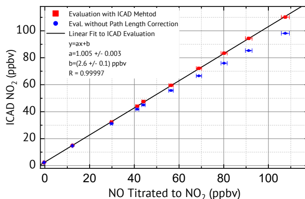
Figure 9. Measurements (spectra recorded with instrument configuration 1) of gas mixtures with different \text{NO}_2 concentration.
