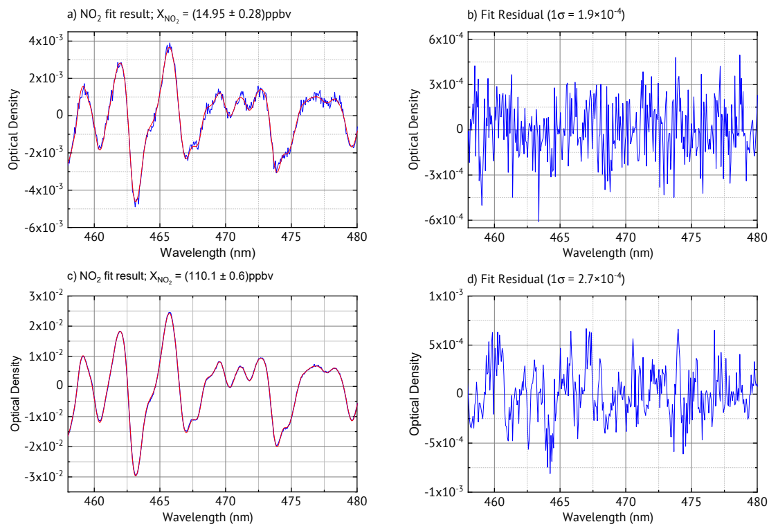
Figure 10. Exemplary ICAD (configuration 1) fit results for gas mixtures of (15.0 \pm 0.3) ppbv a), b) and (110.1 \pm 0.6) ppbv c), d). Panels on the left side show the measured optical density (blue) and the fitted \text{NO}_2 cross section. Panels on the right side show the corresponding fit residuals.
