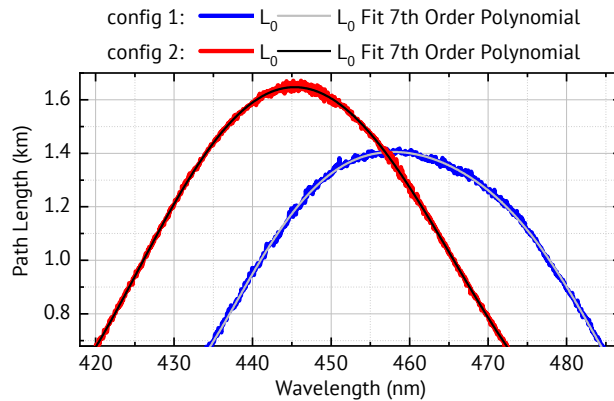
Figure 2. Measured path length L_0 for a zero air filled cavity (only Rayleigh scattering and O_4 absorption see Sect. 4.2) for two instrument configurations, both used in this paper.
