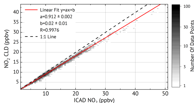
Figure 12. Correlation plot between ICAD NO 2 and CLD/BLC measurements.
