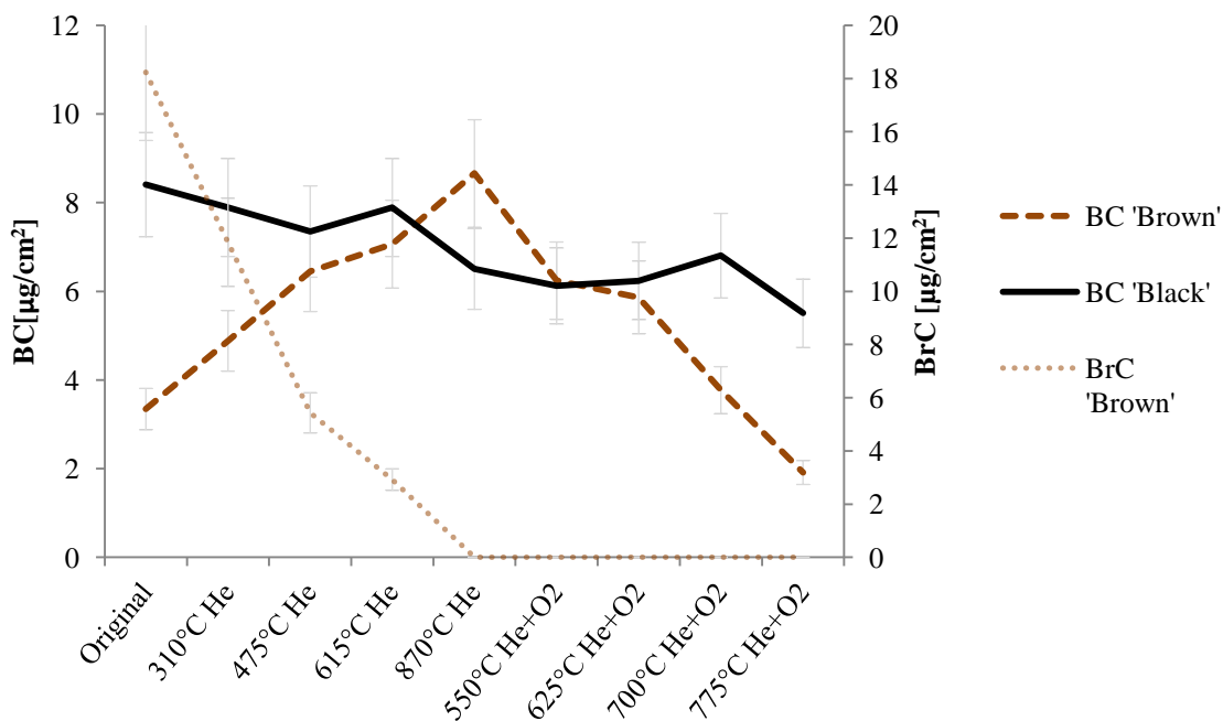
5 | Figure 4: Change of BC and BrC measured with the IS method during the heating according to the NOSH870 protocol measurement for the "black" and the "brown" sample. BC "brown" and BrC "brown" refer to the amount of BC and BrC of the "brown" sample, BC "black" to the amount of BC of the "black" sample. BrC of the "black" sample is below detection limit for the original and the heated samples, respectively. The error bars indicate deviations of \pm 14\% . Laboratory intern test measurements gave variations in this range for filter samples measured in the integrating sphere.
