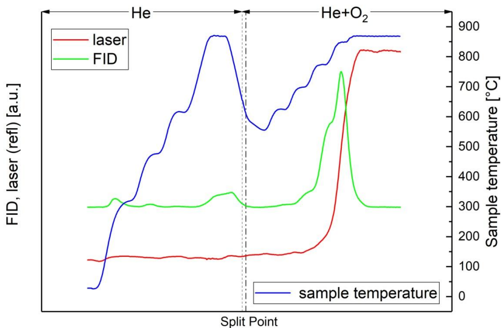
Figure 2: Thermogram of the "black" sample. The blue line is the temperature measured at the position of the sample, the red line the laser reflectance signal and the green line the signal of the flame ionisation detector (FID), which is proportional to the amount of carbon leaving the filter. The split point was set at the point where the laser signal reached its initial value. The FID signal before the split point (broken line) is assigned to OC and after the split point to EC. The dotted line separates the inert and oxidizing phases.
