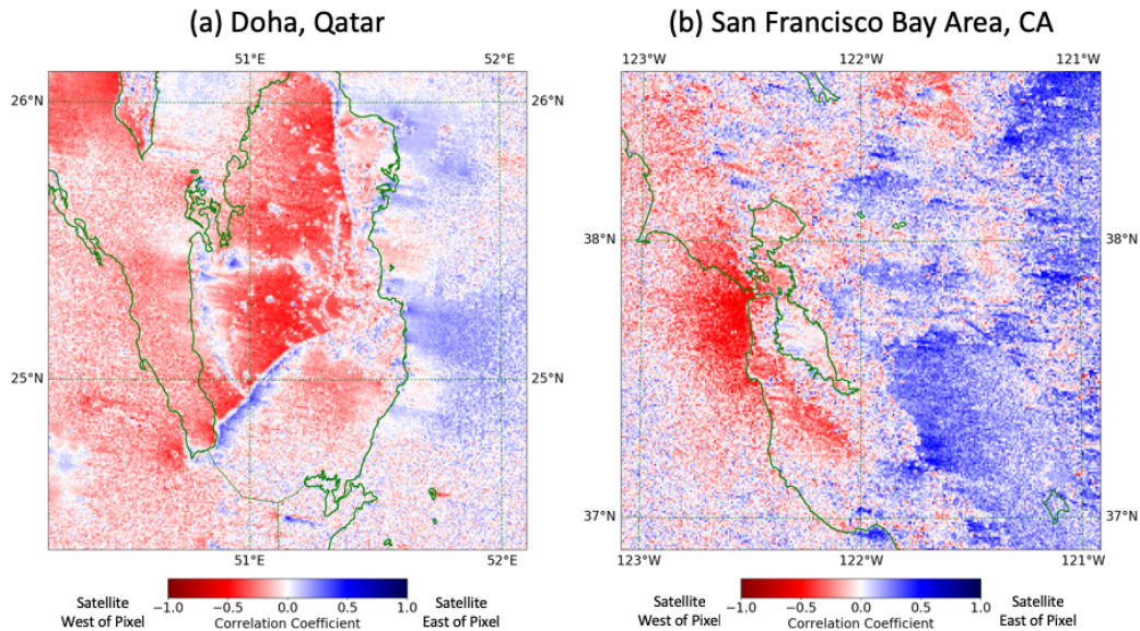
Figure 12: Correlation coefficient on moonless nights (lunar zenith angle > 95^\circ ) for DNB radiance with Directional Satellite Zenith angle ( -70^\circ to 70^\circ ) for (a) Qatar and (b) the San Francisco Bay Area, CA. Negative (red) values indicate that a location appears brighter when viewed from the west (i.e. DNB looking toward the east). Positive (blue) values indicate that a location appears brighter when viewed from the east (i.e. DNB looking toward the west). Values of zero (white) indicate that there is no correlation between the brightness of the pixel and viewing direction.
