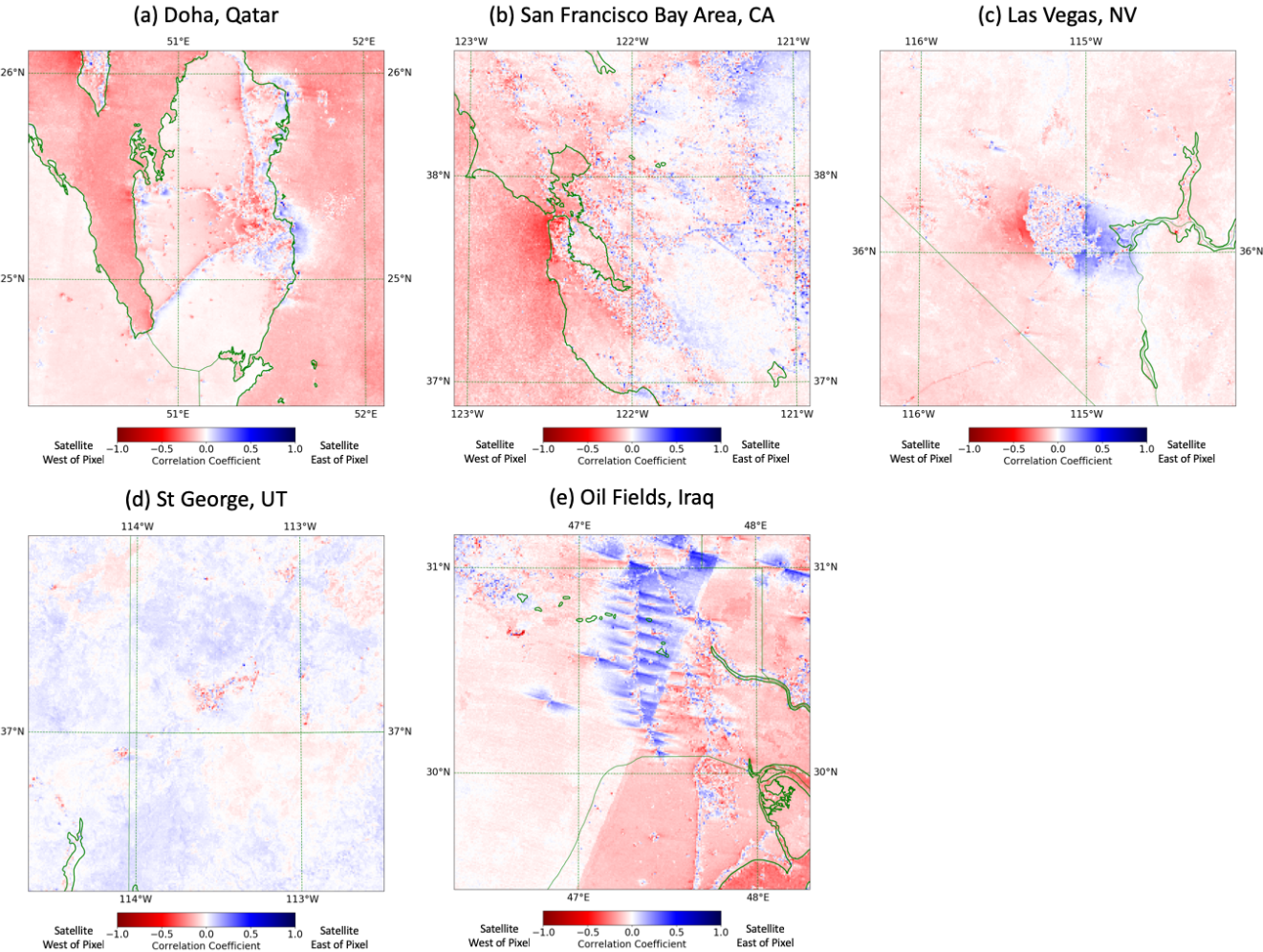
Figure 11: Same as Figure 8 but for DNB radiance vs Directional Satellite Zenith angle (-70° to 70°). Positive (negative) values of Directional Satellite Zenith angle indicate that the satellite is positioned to the east (west) of the location that it is viewing. Positive (blue) values of correlation coefficient indicate that a location appears brighter when viewed by a satellite positioned to the east of that location (i.e. when the DNB is looking toward the west). Negative (red) values indicate that a location appears brighter when viewed by a satellite positioned to the west of that location (i.e. when the DNB is looking toward the east). Zero correlation (white) indicates that a location's brightness is independent of viewing direction.
