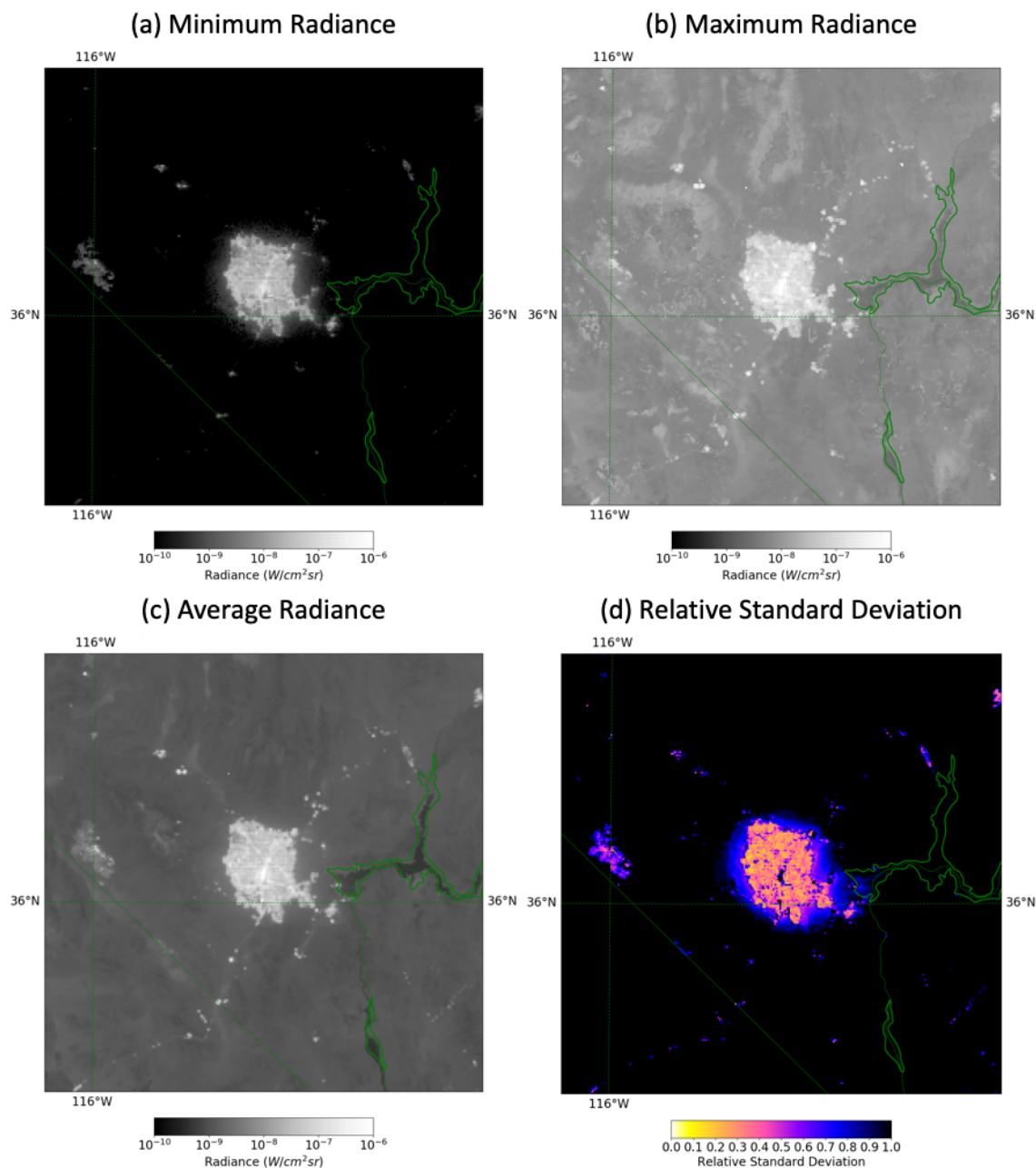
Figure 4: Same as Figure 3 but for Las Vegas, NV, USA.
