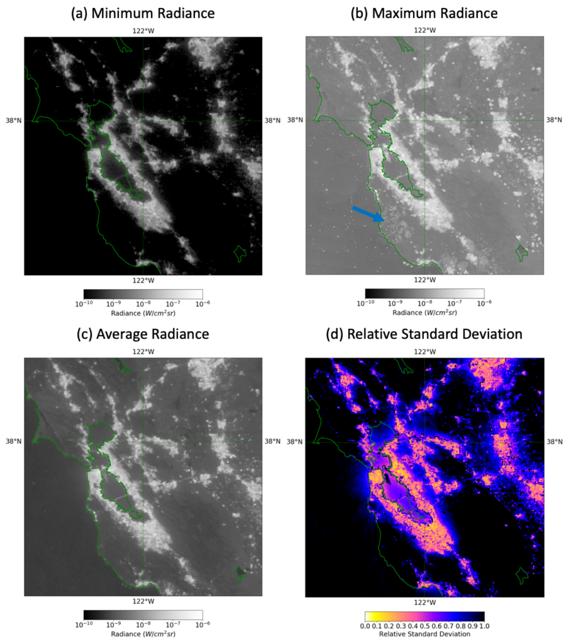
Figure 6: Same as Figure 3 but for the San Francisco Bay Area, California, USA.
