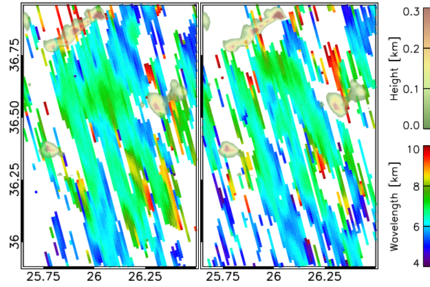
Figure 6. Wavelength, indicated by the lower bar with a colour scale ranging from 4 to 10 km, as derived applying the CWT method to the AIRWAVE TCWV products shown in Fig 4. The left panel shows ATSR-2 orbit 38086 (ascending), the right panel AATSR orbit 2214 (ascending). The height of the ground is also shown (upper bar).
