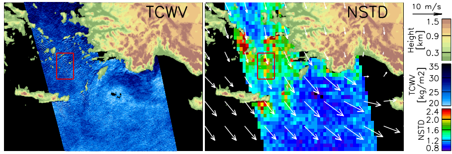
Figure 2. Left panel: AIRWAVE TCWV for 2 Aug 2002, AATSR orbit 2214, ascending. Right panel: corresponding normalised standard deviation. The arrows represent the wind speed (length) and direction, as derived from ERA-Interim products at 1.0^\circ \times 1.0^\circ resolution. The area delimited by the red box is studied more in detail in Fig. 4.
