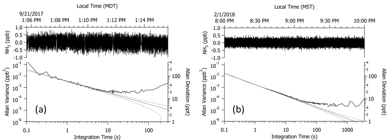
5 Figure 2: 10-Hz measurements collected while overblowing \text{NH}_3 -free air at the inlet tip (a) in flight in the boundary layer near 1.4 km AGL and (b) on the ground in the laboratory. Upper traces represent the raw 10-Hz data collected; lower traces depict the Allan variance in \text{ppb}^2 (left axis) and Allan deviation in ppt (right axis) of the corresponding data set. An offset of -150 pptv was applied to the noise guidelines (gray and dashed lines) in panel (a) to account for differences induced by the vibration applied to the laser objective to reduce motion sensitivity in flight; the vibration was not applied during laboratory tests depicted in panel (b).
