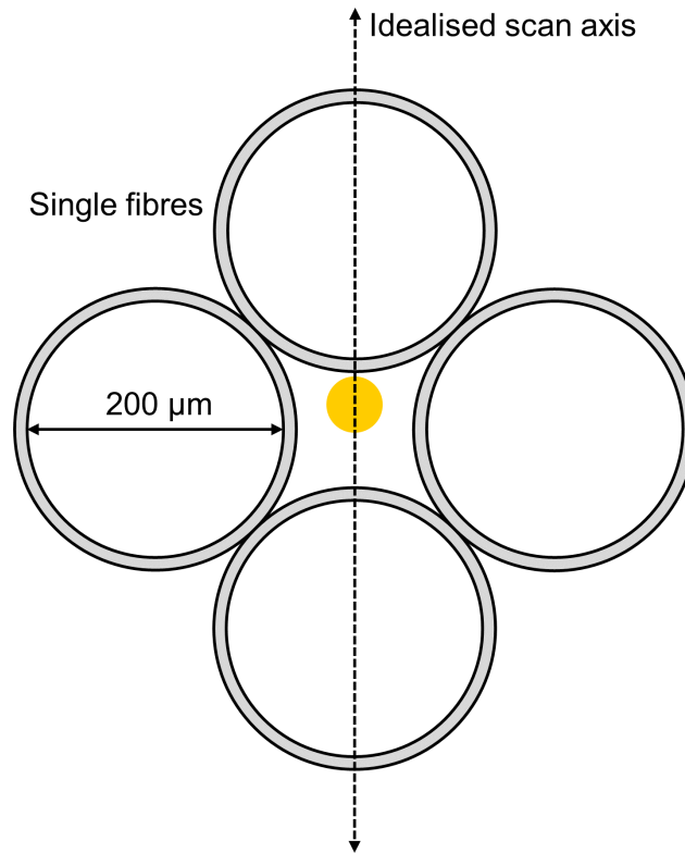
Figure 5. Sketch of the fibre bundle placed in the focal point of the telescope of the MPIC instrument. The grey parts indicate the gladding (additional 20\text{ }\mu\text{m} ) of the fibres. The white circles represent the light-conducting part of the single glass fibres with a diameter of 200\text{ }\mu\text{m} , while the yellow spot indicates the idealised image (neglecting aberration etc.) of the xenon lamp inside the telescope which has a diameter of 7\text{ }\mu\text{m} . Note, that the size of the yellow dot is not shown at the correct scale relative to the fibre diameter and is larger than in reality.
