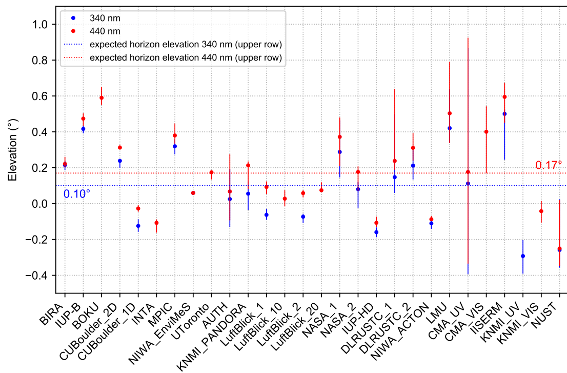
Figure 15. Overview of the retrieved median horizon elevations for all participating instruments at the two different wavelengths. Additionally, the 25%-25th and 75%-75th percentiles are indicated by the lines.
