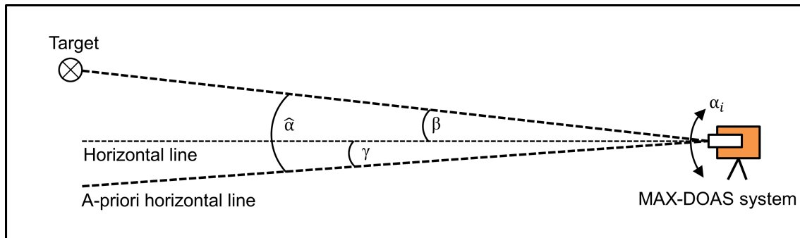
Figure 2. Sketch of the general experimental setup and angle definition used in this study. The horizontal line corresponds to the line of sight of the instrument at 0° elevation.
