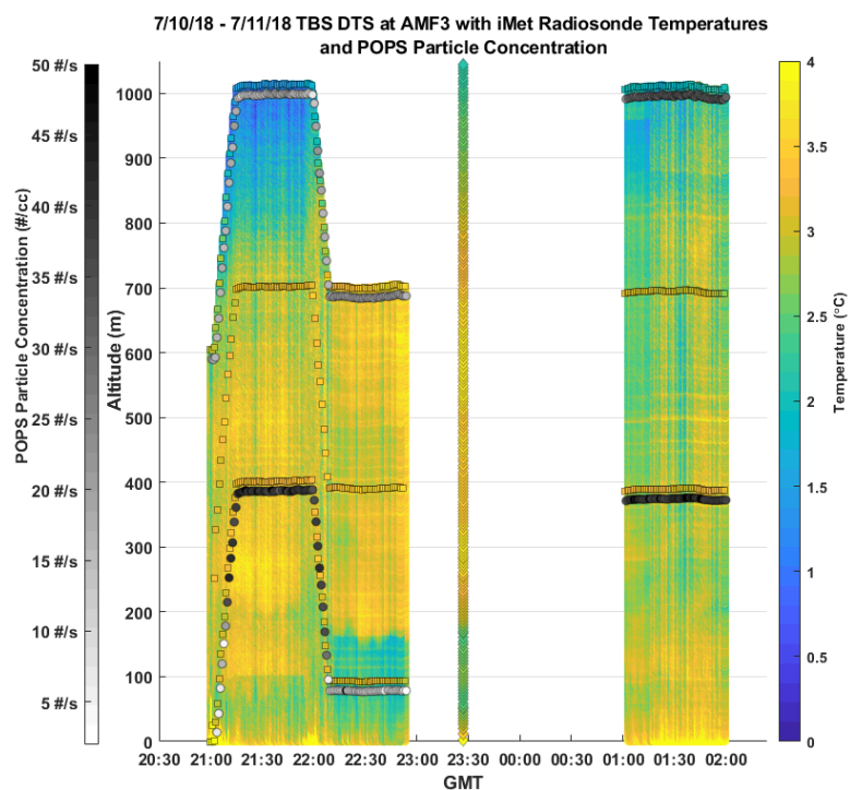
Fig. 2. 7/10/18 – 7/11/18 TBS DTS profiles at AMF3 with TBS iMet temperatures (squares), free-flight radiosonde temperatures (diamonds), and POPS particle concentrations (circles).
