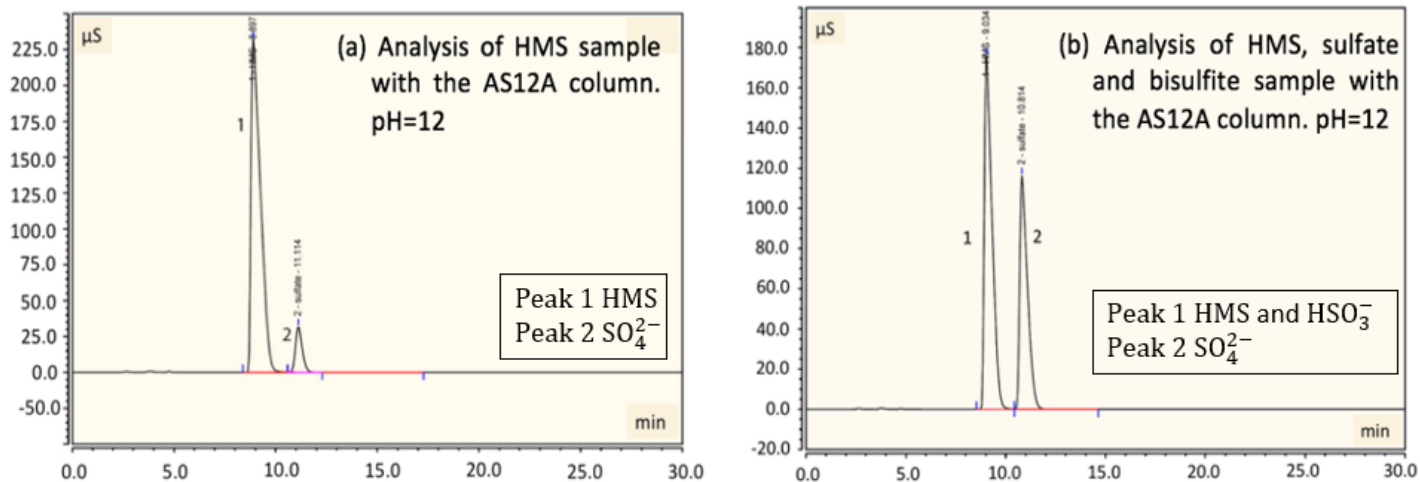
5 Figure 4: Detection and separation of HMS and sulfate using an ion chromatography system with AS12A analytical column and AG12A guard column. (a) A sample of 2 mM of HMS at pH=12 was analysed. A small amount of sulfate is produced due to oxidation by oxygen. The column separates efficiently HMS and sulfate. Peak 1 represents the HMS at 9.6 min and peak 2 represents the sulfate at 11.2 min. (b) A sample of 2 mM of HMS, 2 mM of sulfate and 4 mM of bisulfite at pH=12 was analysed. Peak 1 represents the HMS at 9.0 min and peak 2 represents the sulfate at 10.8 min. The separation of sulfate and HMS is efficient; however, separation of bisulfite and HMS was not possible. Samples were examined at pH=3 and 6 as well with similar separation efficiency as the aforementioned samples.
