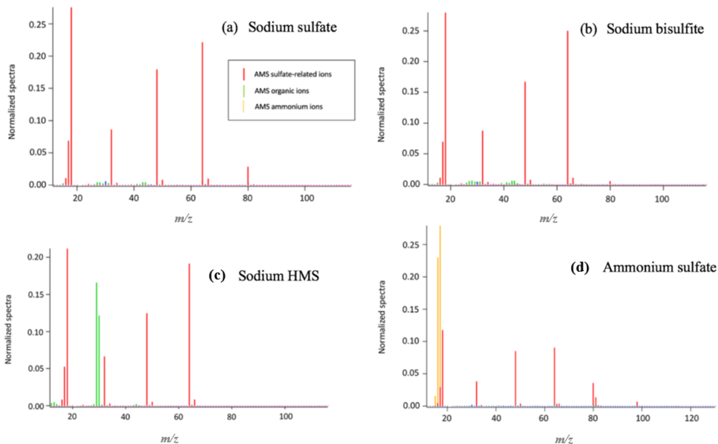
10 Figure 1: Samples analysis using the HR-ToF-AMS. (a) Sodium sulfate fragmentation. The main peaks are \text{SO}^+ ( m/z=48 ) and \text{SO}_2^+ ( m/z=64 ). (b) Sodium bisulfite fragmentation. The spectrum is similar to the sodium sulfate spectrum indicating that their distinction is not possible. (c) Sodium HMS fragmentation. The main differences which allow the distinction among HMS, bisulfite and sulfate is the presence of the organic ions and the absence of the \text{SO}_3^+ ion ( m/z=79.96 ) in the HMS spectrum. (d) Ammonium sulfate fragmentation was used as reference. Similar to (a), (b) and (c) the main ions are \text{SO}^+ ( m/z=48 ) and \text{SO}_2^+ ( m/z=64 ). Ammonium sulfate is also distinguished from HMS due to the presence of the \text{SO}_3^+ ion ( m/z=79.96 ), \text{HSO}_3^+ ion ( m/z=80.96 ) and \text{H}_2\text{SO}_4^+ ion ( m/z=97.97 ). The pH of all samples was 6 and the temperature 25 °C.
