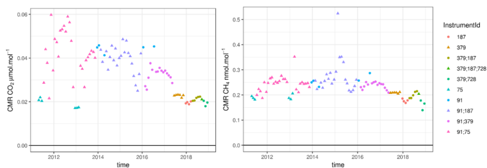
Figure 6: Monthly mean field Continuous Measurement Repeatability (CMR) for CO 2 (left panel), and CH 4 (right panel) estimated over time for the different instruments in operation at the OPE station over the 2011-2018 period. The different instruments are shown in colour and their identifiers are labelled in the key by the right panel. Some months, have several instruments running at the station and these are identified with several labels.
