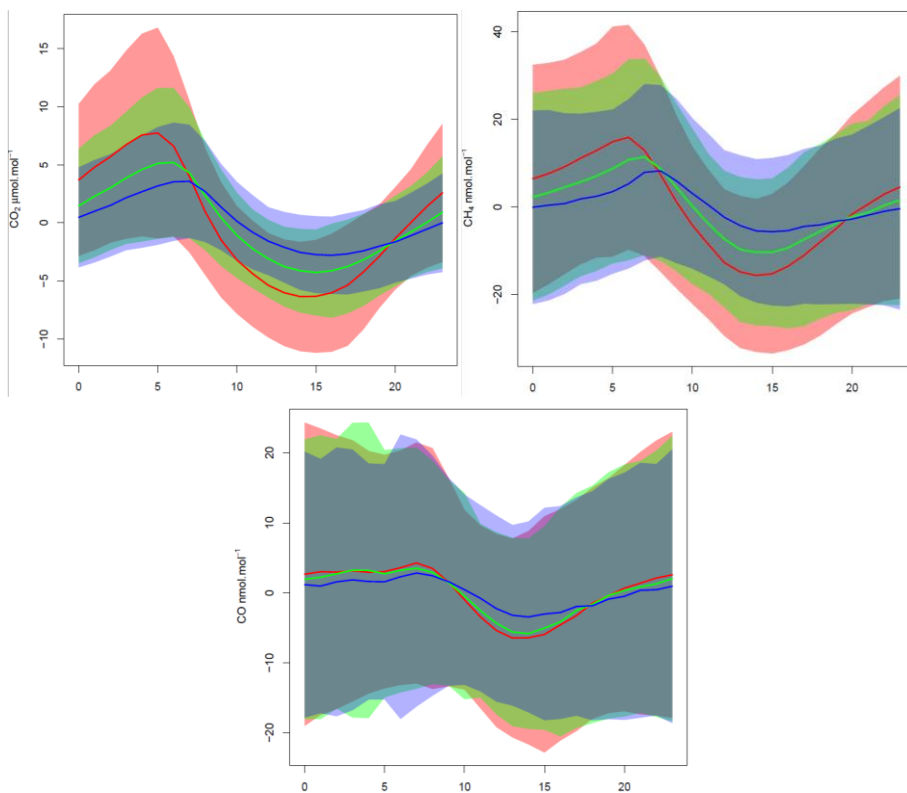
Figure 10 Mean diurnal cycles of CO 2 (top left panel), CH 4 (top right panel) and CO (bottom panel) for the three sampling levels 10m (red), 50m (green) and 120m (blue), computed over the period 2011-2018. The shaded areas correspond to the + and - 1 standard deviations around the mean diurnal cycles.
