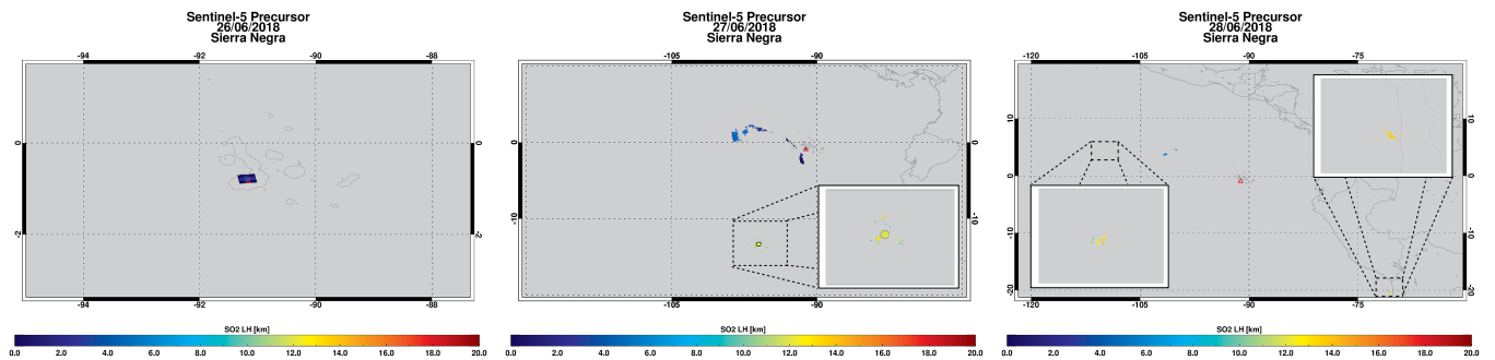
Figure 10. FP_ILM SO 2 LH for the TROPOMI measurements shown in Fig. 9. Note that only pixels with SO 2 VCD \geq 20 DU are shown. The MLS SO 2 measurement of the volcanic plume on 27 June is indicated with a colored circle.
