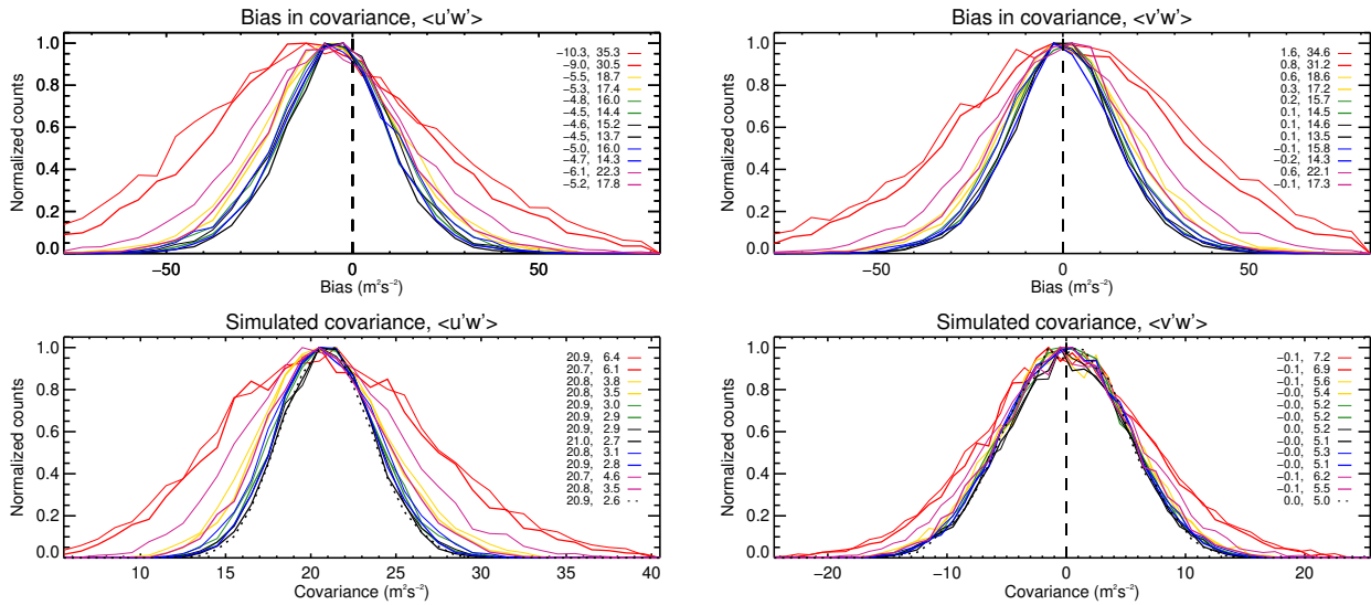
Figure 5. Simulated wind covariance bias distributions for 1 day of integration (upper row) and the simulated covariance distributions (lower row). As discussed in Sect. 3.10, biases are calculated with respect to a “reference” value computed at 2 min resolution at the coordinate system origin. The lower row shows the distribution for the “reference” covariance in a dotted black line, and the “true” covariances in coloured lines. The different line colours in each plot represent different simulated heights, which are a subset of those shown Table 2 (red represents 76 km, yellow 80 km, green 84 km, black 88 km, blue 92 km, and violet 96 km). Thick lines show the distribution for the multistatic case (i.e., by combining data from BP and Mylor), and thinner lines show the monostatic case (i.e., just BP data). The mean and standard deviation evaluated from the samples’ MAD are shown in the left and right columns respectively of the arrays of numbers in each plot figure.
