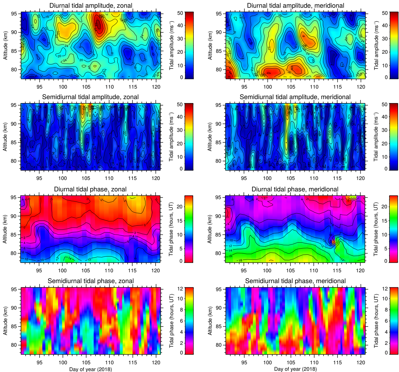
Figure 12. Amplitude of the diurnal (top row) and semidiurnal (second row) tides, and and phase of the diurnal (third row) and semidiurnal (fourth row) tides as measured by the BP-Mylor meteor radar during April 2018.
