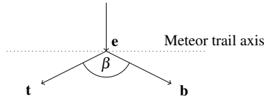
Figure 3. Bistatic meteor geometry. Following the nomenclature in Protat and Zawadzki (1999), \mathbf{t} is a unit vector in the direction of the meteor to the transmitter, \mathbf{b} is a unit vector in the direction of the meteor to the bistatic receiver, and \mathbf{e} is a unit vector that is perpendicular to the meteor trail axis and a bisector of \mathbf{t} and \mathbf{b} . \beta is the so-called “forward scatter” angle.
