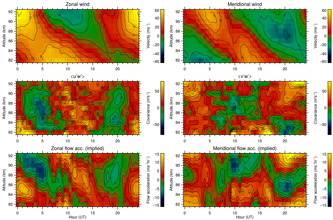
Figure 13. A composite day of the horizontal winds (top row), covariances (middle row) and flow accelerations implied by the covariances (lower row), spanning 5-25 April 2018.
