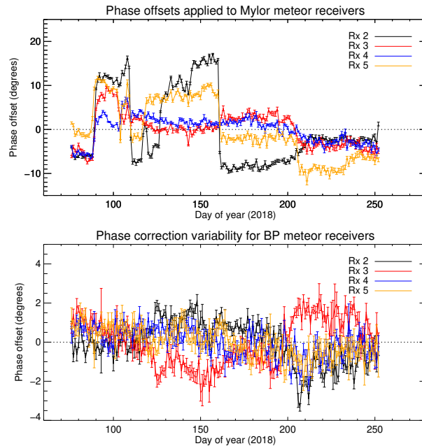
Figure 2. Phase offsets applied to Mylor meteor radar antennas as a function of time (top), and the phase offsets indicated by the Holdsworth (2005) calibration procedure on BP meteor radar data (bottom).
