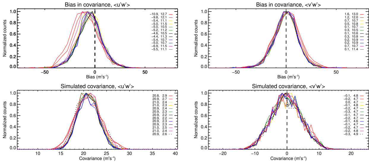
Figure 6. As per Fig. 5, but for 10 days of integration.
