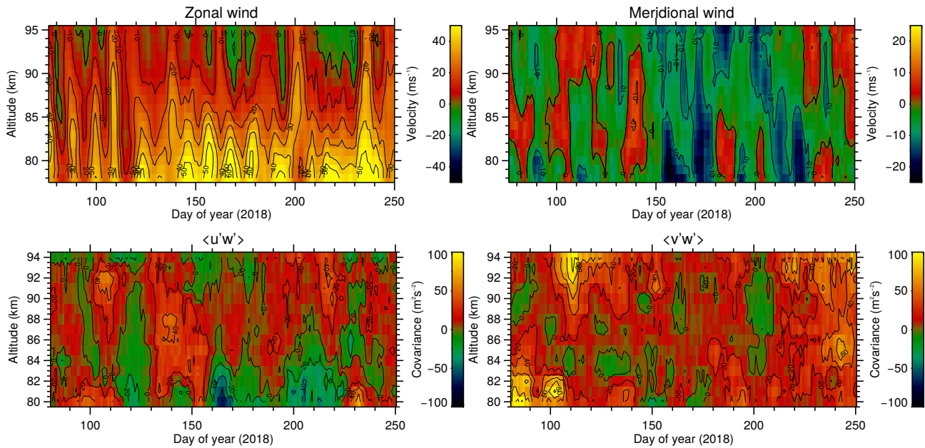
Figure 10. Mean horizontal winds (top row) and the \langle u'w' \rangle and \langle v'w' \rangle covariance components measured using the BP-Mylor link between 17th March and 9th September 2018. As discussed in Sect. 4.1, the winds shown correspond to a 10-day moving average of the hourly-averaged winds with tidal components removed, and the covariances have been evaluated over 10-day windows, with a gap of 2 days between the centres of adjacent windows.
