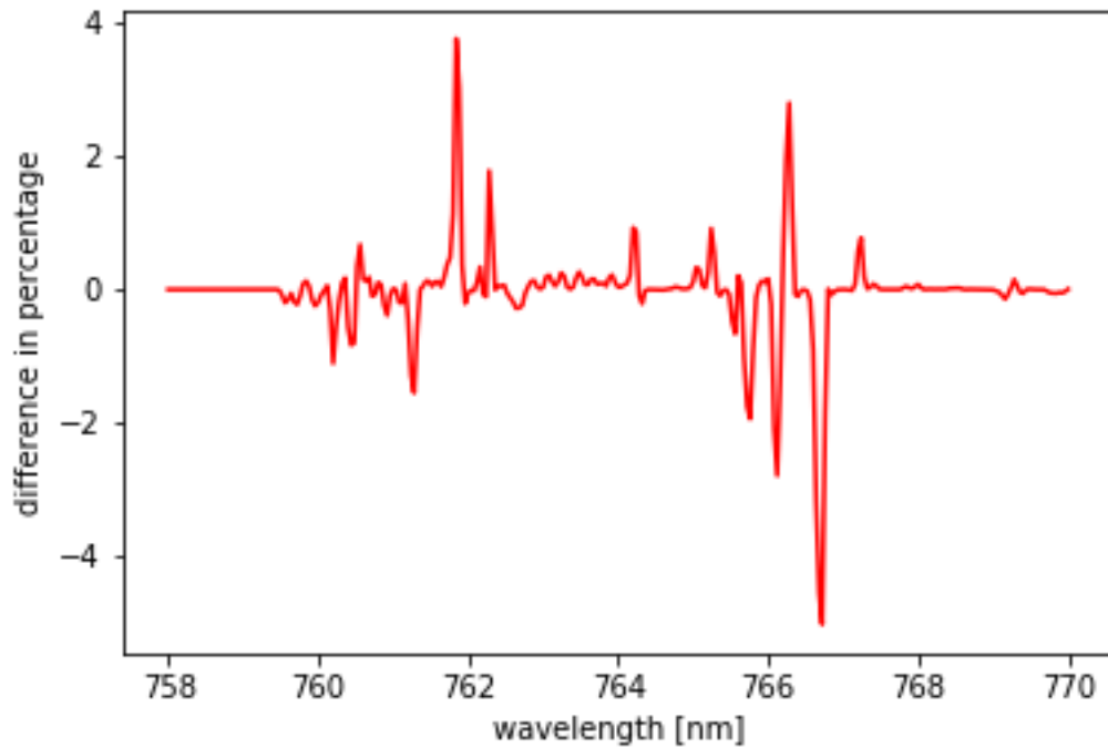
Figure 1: The difference (reported as a percentage) between the two convolution processes, one with Io correction and the other without.
