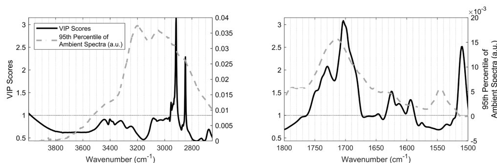
10 Figure 2. Variable Importance in the Projection (VIP) scores generated from the calibration models, as a weighted sum of the functional groups (see Supplementary Material, Sect. 12, for calculation). An ambient spectrum is overlaid for comparison (95th percentile of all ambient spectra).
