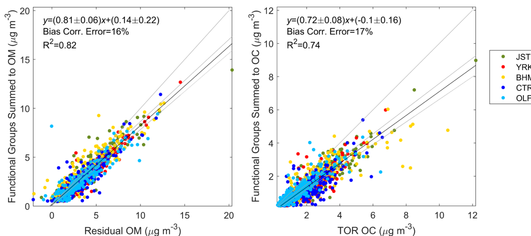
5 Figure 3. Scatter plots of predicted functional group OM and OC concentrations versus reference measurement concentrations. Left: reference values are residual OM concentrations; FT-IR OM MDL=0.38 \mu\text{g m}^{-3} . Right: reference values are TOR OC concentrations; FT-IR OC MDL=0.19 \mu\text{g m}^{-3} . Site abbreviations: JST = Jefferson Street, Atlanta, GA; YRK = Yorkville, GA; BHM = Birmingham, AL; CTR = Centreville, AL; OLF = Outlying Landing Field (near Pensacola), FL.
