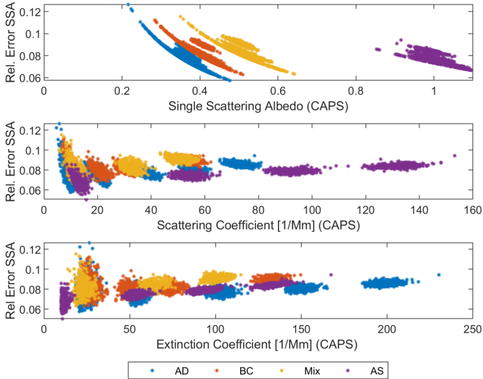
515 Figure 13 Relative error of the Single Scattering Albedo (SSA) derived from CAPS measurements as function of the derived SSA (top-), the scattering coefficient (middle-), the extinction coefficient (base-plot).
