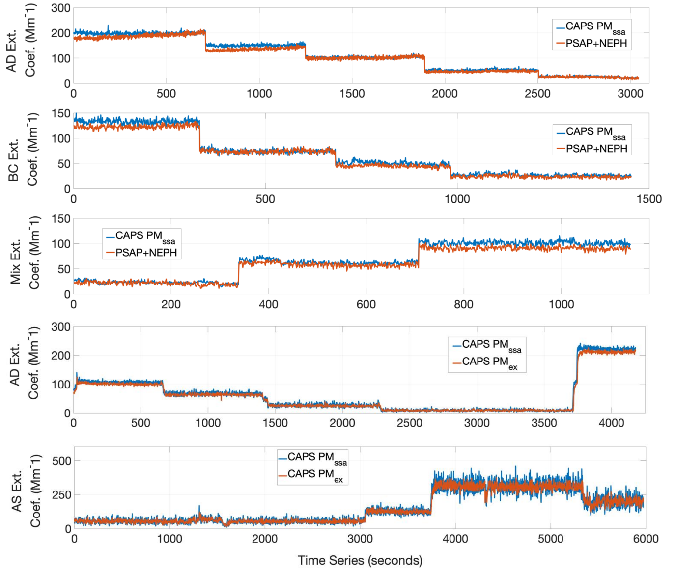
Figure 4. Time series of the parallel measured extinction coefficients by the different instruments. Instruments used: CAPS PM ex , CAPS PM ssa and the sum of absorption- and scattering coefficients measured by PSAP and NEPH as noted in the legend for the individual subplots. The test aerosols used are noted in the caption of the y-axis of the individual subplots.
