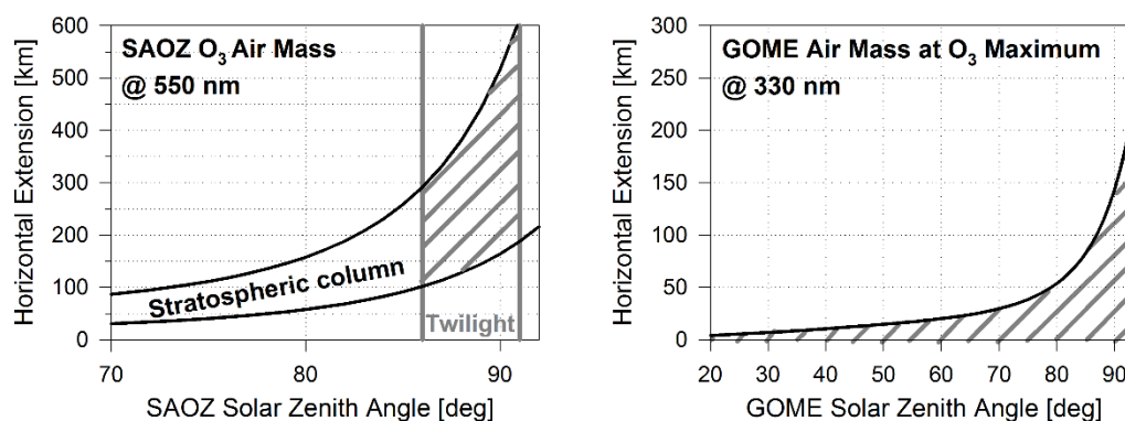
10 Figure 4: Estimated horizontal extension of the ozone air mass probed by the zenith-sky UV-visible spectrometer from 70° to 92° SZA (calculation based on SAOZ settings in the Chappuis band at 550 nm). The shaded area shows the air mass extension during the twilight period. Reproduced from Lambert & Vandebussche (2011).
