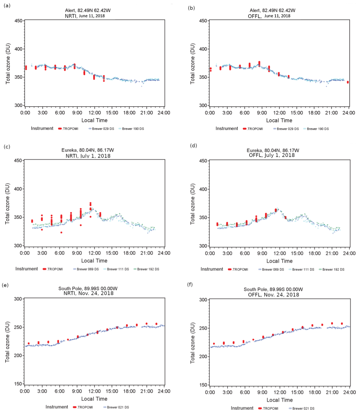
Figure 9: The diurnal variation of the TOC (in DU) measured by TROPOMI (left panels NRTI product and right panels OFFL product) and Brewer spectrophotometers at three high latitude Northern and Southern stations that are part of the Canadian Network. The maximum distance for the co-locations is 10 km.
