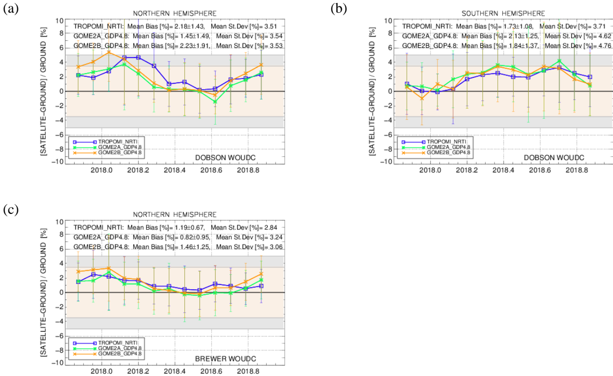
Figure 14: As for Figure 12 but for the time series of the percentage differences between TROPOMI NRTI (blue line), GOME2A (green line) and GOME2B (orange line), the two latter processed with the GDP4.8 algorithm.
