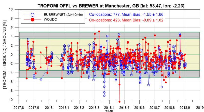
10 Figure 3: The time series of the comparisons between TROPOMI and GB TOC measured at Manchester, Great Britain. Blue circles: individual GB measurements with temporal maximum difference of 40 min from the TROPOMI measurements (Eubrewnet) are used, red dots: TROPOMI compared to daily means of the GB measurements (WOUDC). Both data sets refer to the same time period.
