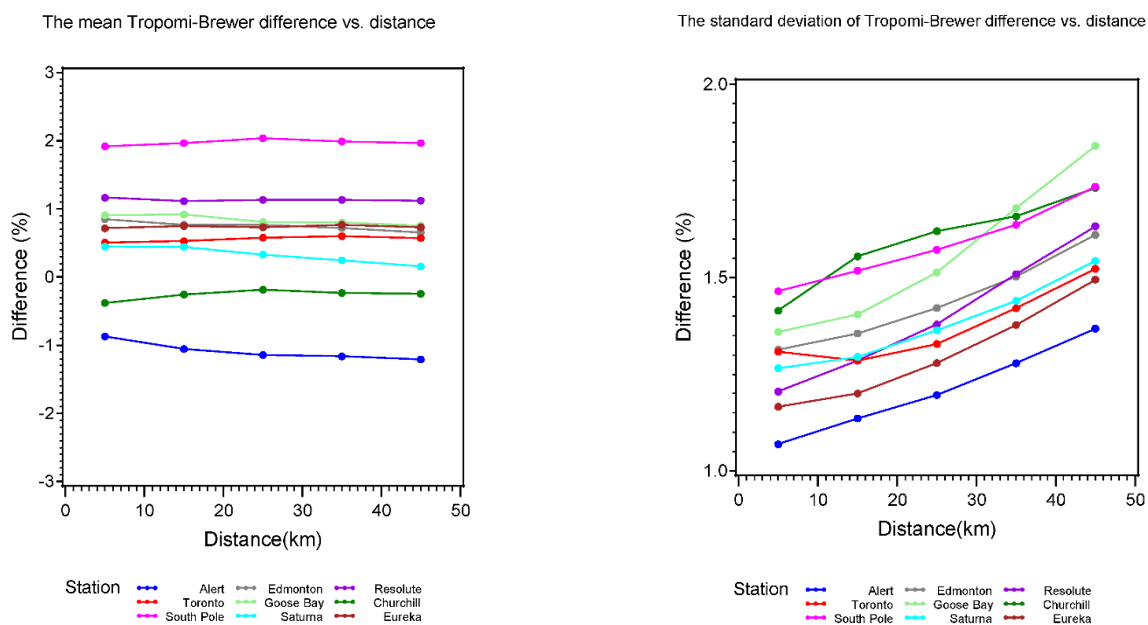
Figure 1: The percentage difference (left panel) and the standard deviation (right panel) of the TROPOMI OFFL TOC compared to GB measurements, versus the co-location search radius (in km) for nine Brewer stations of the Canadian Network (See Table S. 4 in the Supplement for details on these stations).
