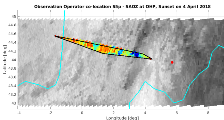
15 Figure 5: Illustration of the co-location procedure for TROPOMI vs. SAOZ measurements, in this case for a sunset SAOZ measurement at the Observatoire de Haute Provence (France) in local spring. The red disk marks the instrument location. The black polygon is the observation operator, i.e. the parametrized extent of the actual twilight measurement sensitivity. The grey background is the TOC measured in a temporally co-located TROPOMI orbit (#2456) and the coloured pixels are those that fall within the observation operator, i.e. those that are averaged before being compared to the SAOZ measurement.
