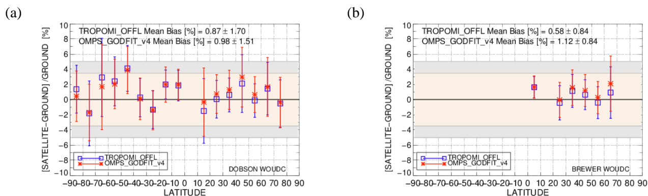
Figure 13: The latitudinal dependency of the percentage differences between the two satellite sensors' TOC (TROPOMI OFFL and OPMS) processed with the GODFIT v4 algorithm, and Dobson (panel a) and Brewer (panel b) GB measurements from WouDC. The symbol colors are as in the previous Figure.
