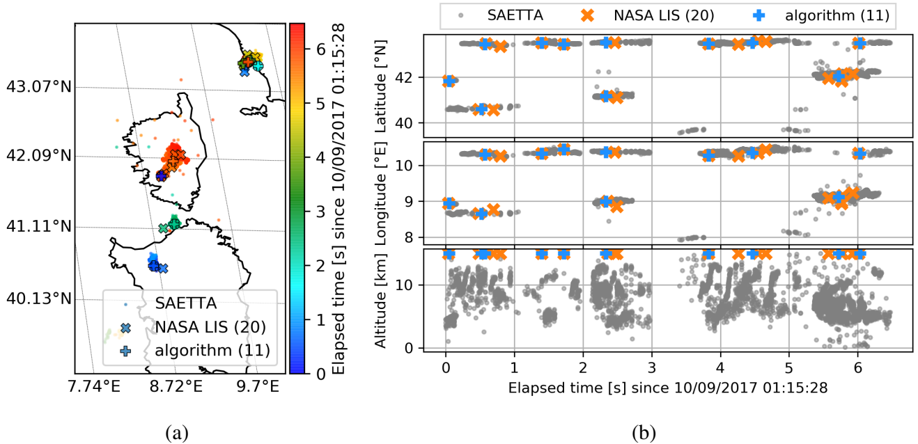
Figure 3. The map (a) and time series (b) of SAETTA observations and the mean flash positions based on the NASA LIS algorithm and our developed algorithm for one situation on Sept. 10, 2017. The numbers in parentheses in the legend indicate the number of identified flashes (both algorithms analyzed the same LIS events). Colors in (a) represent the elapsed time from the initial lightning activity. Note: Flash altitudes in (b) are not known for ISS-LIS flashes but arbitrarily plotted at 15 km.
