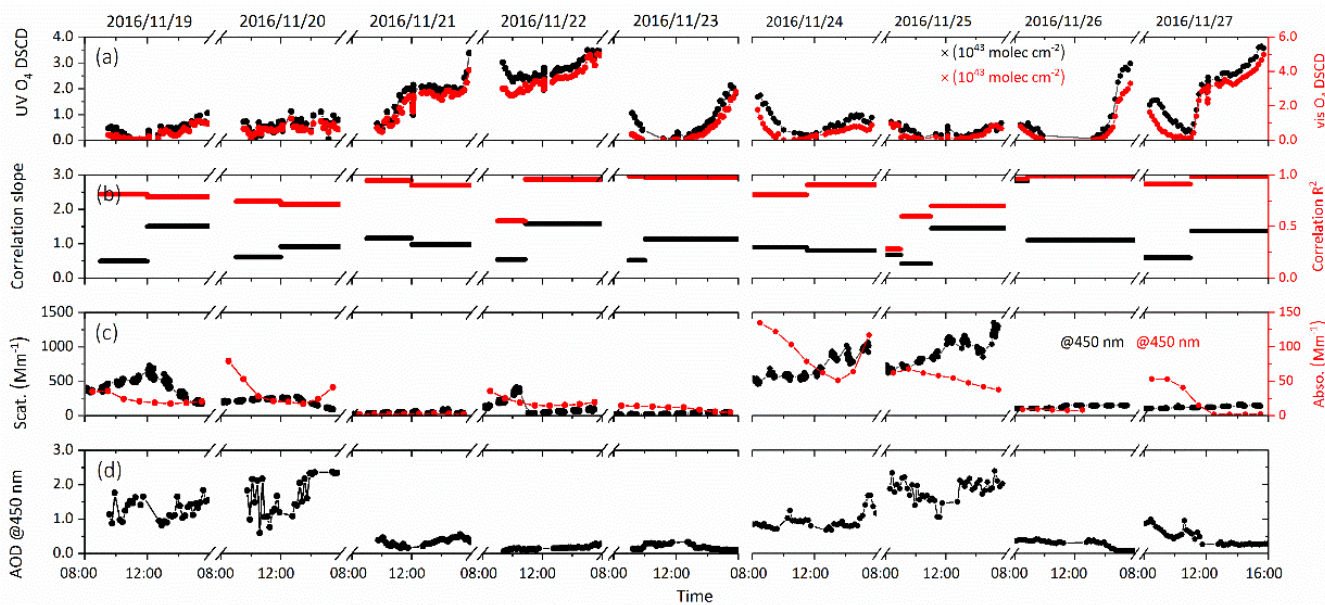
Figure 7. Time series of O 4 absorptions and aerosol optical properties at Gucheng, Hebei from 19 to 27 November 2016: 320 (a) UV and visible O 4 DSCDs, (b) correlation slopes and R 2 between O 4 DSCDs at 360.8 and 477.1 nm, (c) \sigma_{\text{sca}} and \sigma_{\text{abs}} at 450 nm, (d) AOD at 450 nm retrieved by MAX-DOAS.
