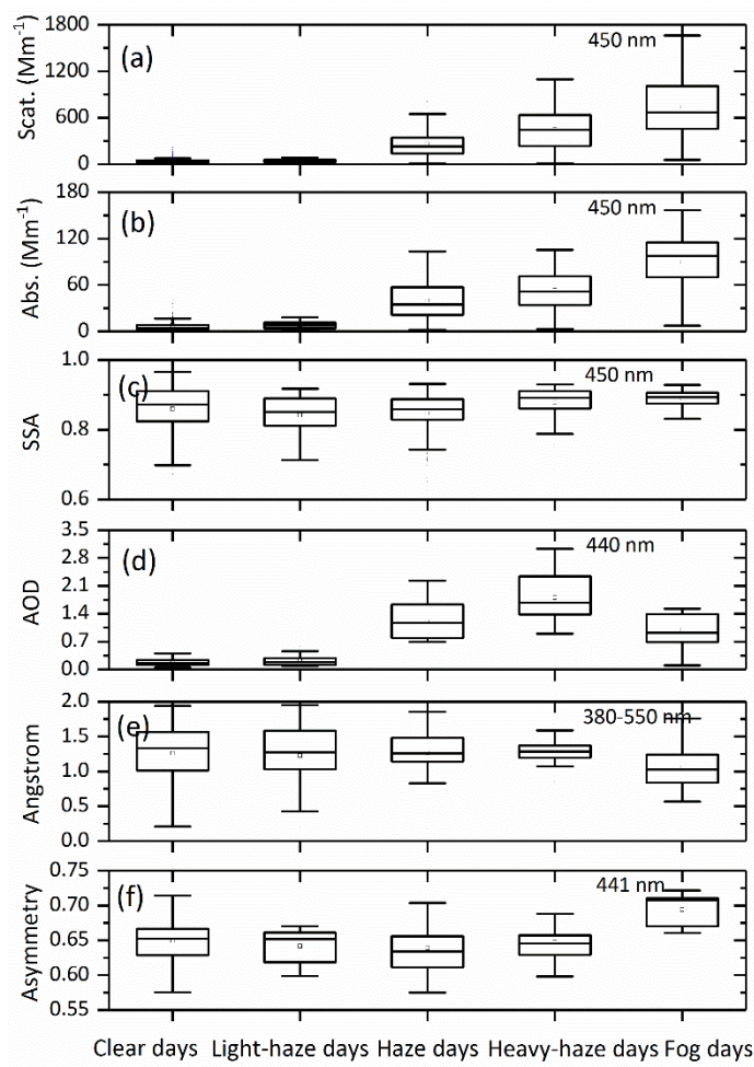
280 Figure 6. Box plots of the statistics on aerosol optical properties under different weather conditions: (a) \sigma_{\text{sca}} , (b) \sigma_{\text{abs}} , (c) SSA, (d) AOD, (e) Angstrom and (f) Asymmetry.
