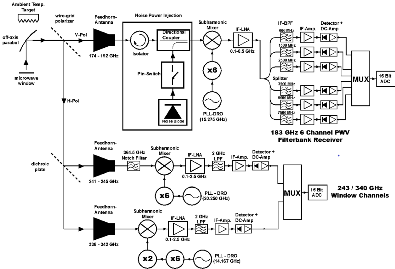
Figure 2. Block diagram of MiRAC-P.
