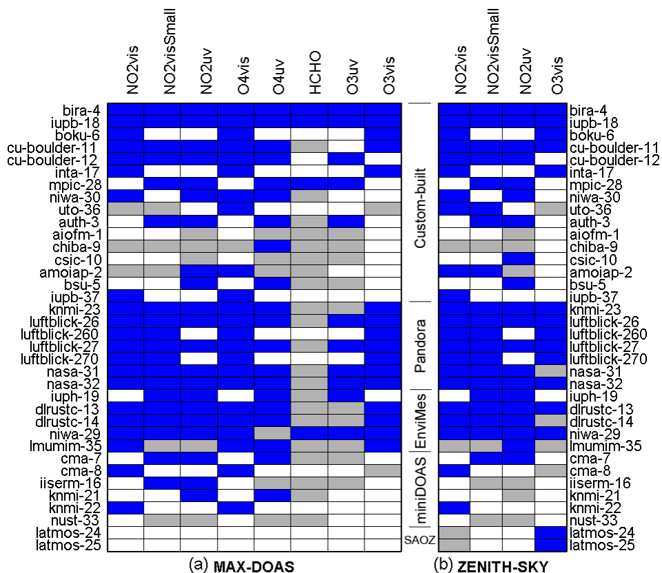
Figure 8. Instrument data sets selected to build the median MAX-DOAS reference (a) and zenith-sky (b) data sets. Blue marks the data sets included in the median, grey marks the data sets not included and white the ones not available. Note that the instruments are grouped according to their specific design as custom-built, Pandora, EnviMes, mini-DOAS or SAOZ.
