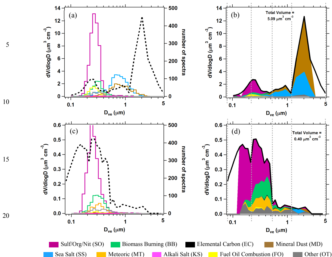
Figure 2: Quantification of PALMS particle classes. (a,c) Raw PALMS counts for different particle classes (colors) overlaid on the aerosol volume size distribution (dashed black). (b,d) For each diameter bin, the fractional contributions of each PALMS particle class are applied to the total volume. Vertical dashed lines define four broad diameter bins that are used to generate concentration products at higher time resolution (see text). The upper panels are from 39 min of sampling at low altitude over the Gulf of Mexico and contain influences from the marine boundary layer, long range mineral dust transport, and lower tropospheric pollution. The bottom panels represent the remote upper troposphere with minor influences from continental and stratospheric sources, sampled over 27 min.
