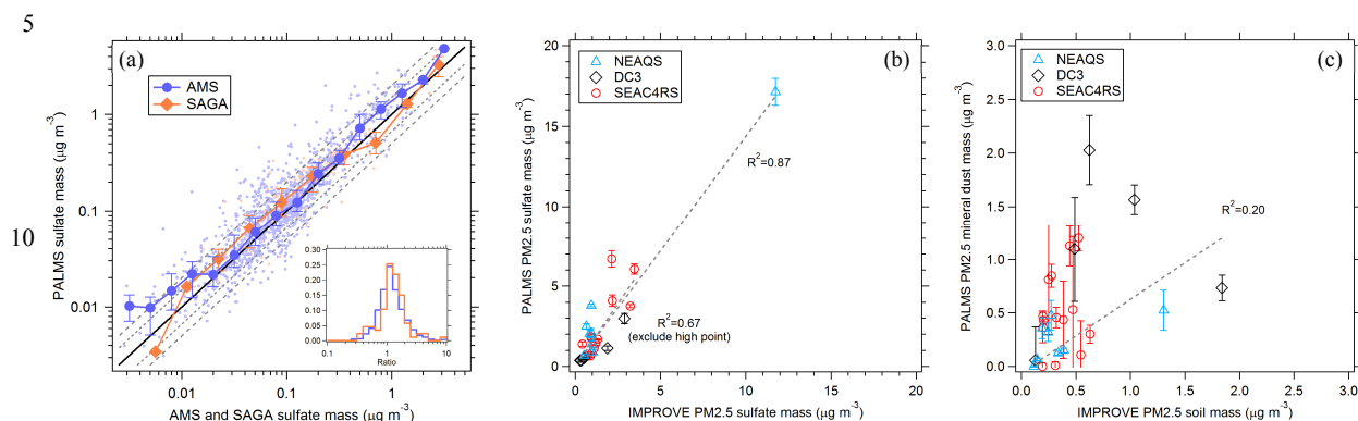
Figure 8. Comparison of PALMS with other speciated aerosol mass measurements. (a) PALMS derived sulfate mass at 3 min time resolution compared to co-located AMS and SAGA filter samples during the ATom-1 airborne campaign. Sea salt sulfate ( 0.25\text{xNa}^+ ) is subtracted from SAGA data. SAGA filters taken over an altitude range >3 km are excluded. Small points are 3-min averages (blue) or represent one SAGA filter measurement (orange). Large symbols are medians with interquartile error bars. The solid black line is 1:1, and grey dashed lines are 1:1.5 and 1:2. The inset graph is a histogram of PALMS ratio to AMS or SAGA for all individual samples. PALMS sulfate (b) and mineral dust (c) mass are compared to nearby IMPROVE ground station data for three airborne campaigns. Each point is the average of airborne data for non-targeted flight segments in the continental boundary layer within 0.5^\circ latitude and 1^\circ longitude of an IMPROVE site that reported data that day. IMPROVE data are 24 h averages, and airborne segments are typically \sim 3 –30 min duration during daytime. Error bars are estimated statistical uncertainty calculated as described in Appendix A. Dashed lines are weighted linear fits.
