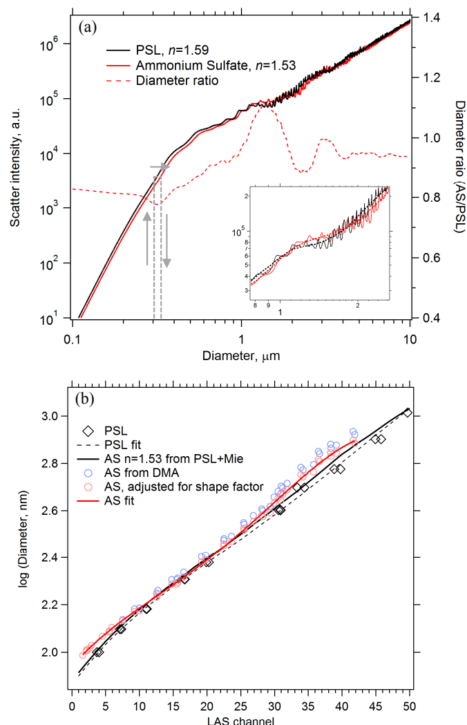
Figure 4. Using Mie theory to translate the response of an optical particle spectrometer between particles of different refractive index. (a) Calculated scatter intensities at \lambda=663 nm for PSL and effluoresced ammonium sulfate (AS) particles in the LAS instrument. PSL diameters are translated into ammonium sulfate diameters of the same scatter intensity using the Mie response curves, shown conceptually with grey arrows. The diameter ratio is plotted on the right axis. Smoothing must be applied to the Mie curves (inset a, dashed) in order to yield unique diameter translations. (b) A calibration curve derived from PSL particle standards (dashed black) is translated into an ammonium sulfate calibration curve (solid black) using Mie theory. Size-selected AS particles yield a directly measured AS calibration curve (solid red) to compare with the PSL-derived AS calibration curve.
