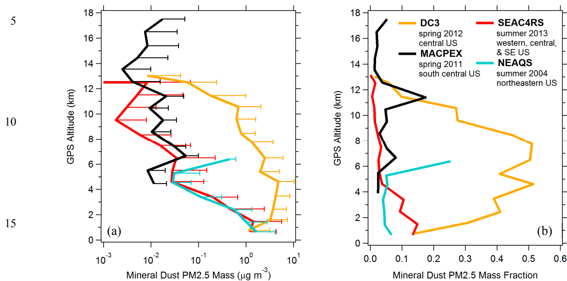
Figure 9. Vertical profiles of PALMS mineral dust mass (a) and mass fraction (b) over the continental US for D_{ve} > 0.1 \mu\text{m} . Lines are campaign average concentrations binned at 1 km intervals from products generated at native resolutions of 3 min (SEAC4RS, DC3, NEAQS) or 5 min (MACPEX). Biomass burning plumes and clouds are excluded. By truncating the size range using a typical cyclone impactor transmission curve with D_a(50\%) = 2.5 \mu\text{m} ( http://www.urgcorp.com/ ), these mass concentrations are equivalent to a PM 2.5 measurement. The MACPEX size range is limited by the optical particle spectrometer to D_{ve} < 1.5 \mu\text{m} . Positive error bars are one standard deviation.
