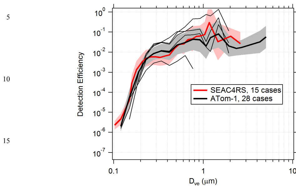
Figure 6. Detection efficiency curves for the PALMS instrument in flight. Detection efficiency was calculated for several cases, identified as clean flight segments when the particle data rate was not actively limited by software or hardware. Thick lines and shading are geometric means and standard deviations over all cases. Higher efficiencies for D_{ve} > 3 \mu\text{m} during ATom are partly due to addition of a virtual impactor upstream of PALMS. Thin black lines are five individual cases during one ATom-1 flight. Variations in altitude, particle composition, inlet performance, and unknown factors result in detection efficiencies that vary by > \times 10 within and between flights. The lowest thin line was a case where a buildup of aerosol material on the pressure reduction orifice altered particle trajectories inside the inlet.
