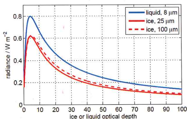
20 Figure 2. Radiances extracted from the liquid (blue) and ice (red) look-up tables for a range of different optical depths, all calculated for a solar zenith angle of 30^\circ and at the visible 440 nm wavelength over a surface of albedo 0.05. The numbers in the legend are values of liquid effective radius and ice effective diameter.
