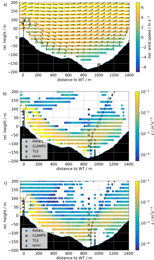
Figure 14. In (a) the coplanar wind field reconstruction from RHI#1 and RHI#2 from averaged RHI scans between 0400 UTC and 0430 UTC is shown. The arrows show the wind vectors projected onto the RHI plane as retrieved with the coplanar method (Wildmann et al., 2018a). The colormap is scaled with the horizontal wind component of the projected wind vector. (b) and (c) show dissipation rates as estimated from CLAMPS, TLS and towers 20/trSE_04 and 25/trSE_09 on scans by RHI#1 (b) and RHI#2 (c) for the same time period.
