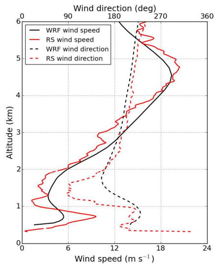
Figure B1. Wind speed and wind direction up to 6 km as an average from 0300-0330 UTC from WRF simulations ( black lines ) and from the radiosonde-radiosonde (RS, red lines ) launched at 0255 UTC on 14 June 2017.
