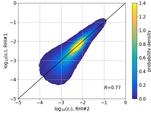
Figure 9. Comparison of all estimations estimates of \varepsilon in the RHI plane for 9-15 June 2017 between RHI#1 and RHI#2. The color scales represent the probability of occurrence of a measurement point. The black line is the line of identity. Data points with probability density below 0.02 are not shown.
