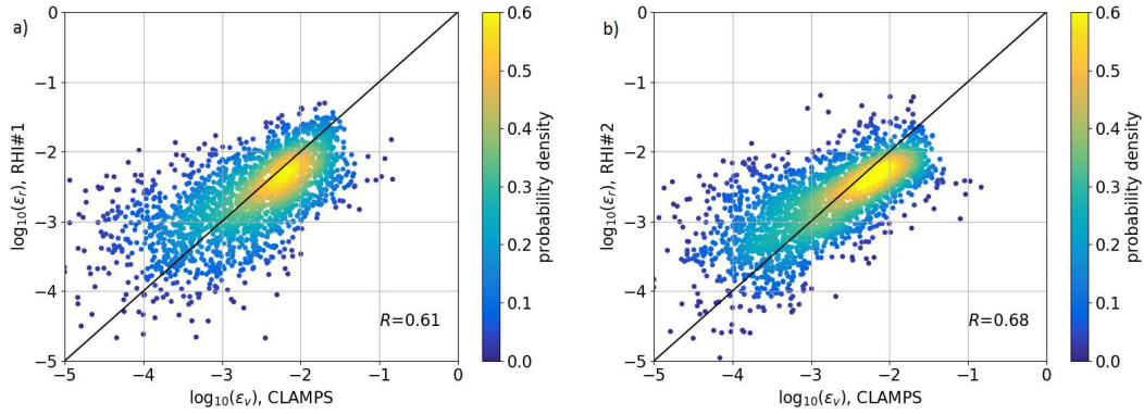
Figure 8. Comparison of all estimates of \varepsilon in the vertical profile over the valley from 9-15 June 2017 from RHI#1 (a) and RHI#2 (b) against the Halo system. The color scale represents represent the density of probability of occurrence of a measurement point. The black line shows identity.
