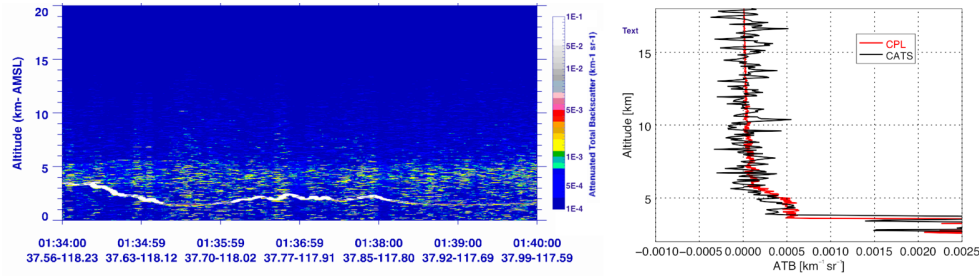
10 Figure 5: The CPL curtain plot of ATB centered around the 01:37 UTC coincident point from the 7-8 August 2015 CCAVE flight (Left). The mean ATB profiles from CATS and CPL during this under flight (right).
