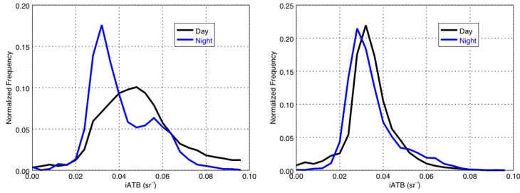
5 Figure 4: Distributions of CATS strongly scattering, rapidly attenuating opaque cirrus iATB distributions from V2-01 (left) and V3-00 (right). These plots demonstrate the CATS daytime calibration method using calibration transfer from the nighttime calibration.
