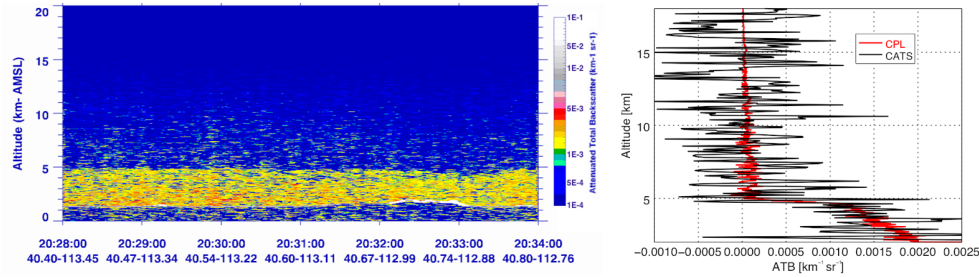
15 Figure 6: The 20 August 2015 CATS/CPL coincident flight. The CPL 70 km coincident segment curtain plot (left) was used to compute the mean ATB profile (right) from CPL along the same path as CATS. The CATS and CPL data show good agreement despite higher noise levels in the CATS profile due to daytime retrieval limitations.
