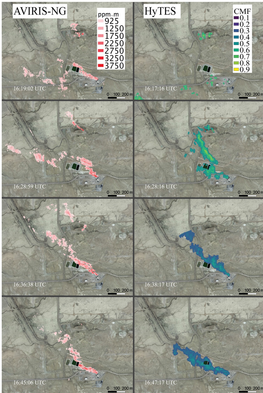
5 Figure 1: Methane plume over a venting shaft in the Four Corners region, observed from four individual airborne instrument AVIRIS-NG overpasses (2.8 m spatial resolution) at 7-9 minutes apart on April 22 nd , 2015 between 16:19:02 and 16:45:06 UTC (left) compared with observations from HyTES overpasses (2.3 m spatial resolution) in the similar interval between 16:17:16 and 16:47:17 UTC (right). The background is from Google Earth imagery.
