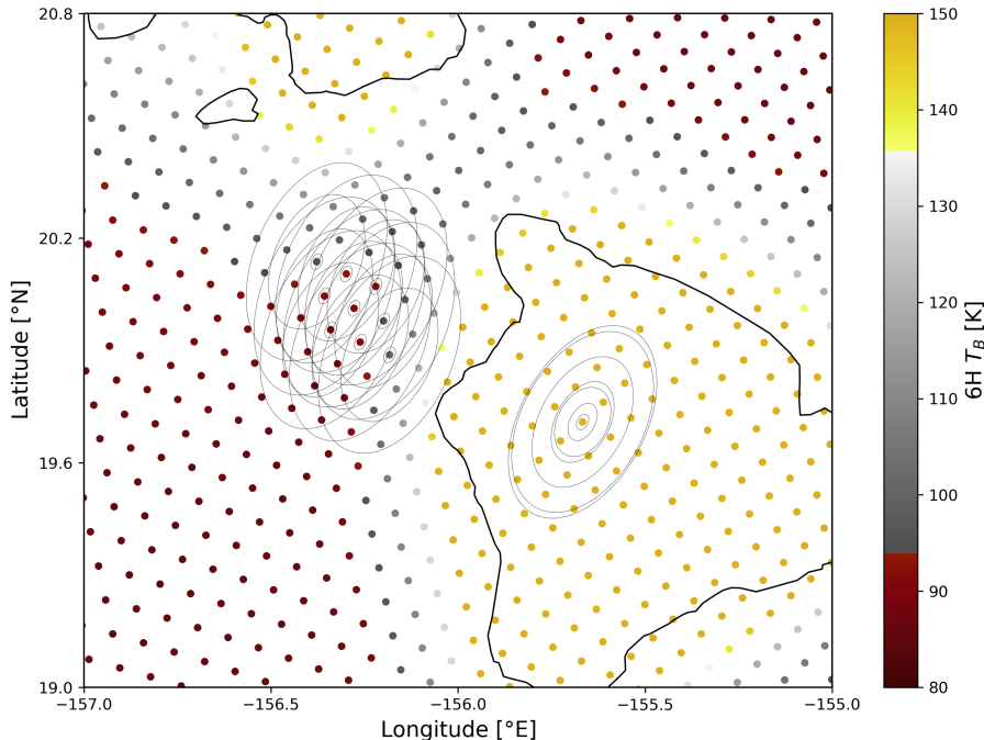
Figure 1. An example of FOV sizes and measured T_B at the 6H channel near the Island of Hawai'i, from an AMSR2 orbit on September 21, 2016. The T_B s at 6H are shown in coloured dots, with the HPBW given at all AMSR2 frequencies for one observation centre viewing the island itself. The HPBW is outlined for three frequencies only (6, 10, 89GHz), for three consecutive observation centres along- and across-scan just west of the island, so as to view the spatial overlap without too much clutter.
