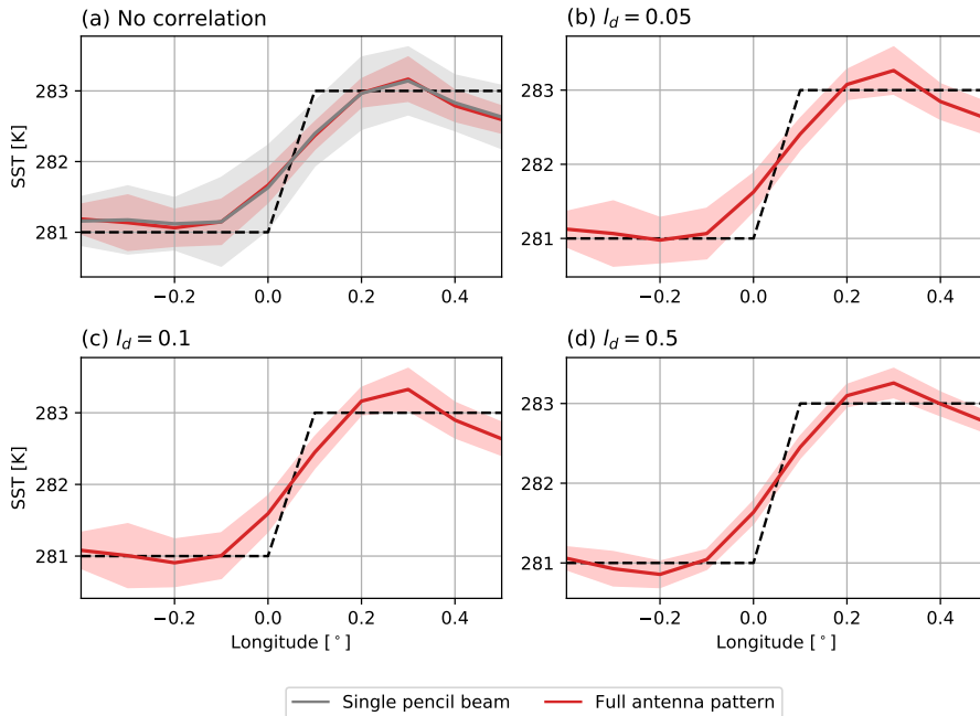
Figure 11. A synthetic scene as Fig. 3, but with the background defined by a step function in SST, shown by the dashed line and consistent across latitudes. The shaded areas represent the spread of retrieved SST in the latitudinal direction and the solid lines the means.
