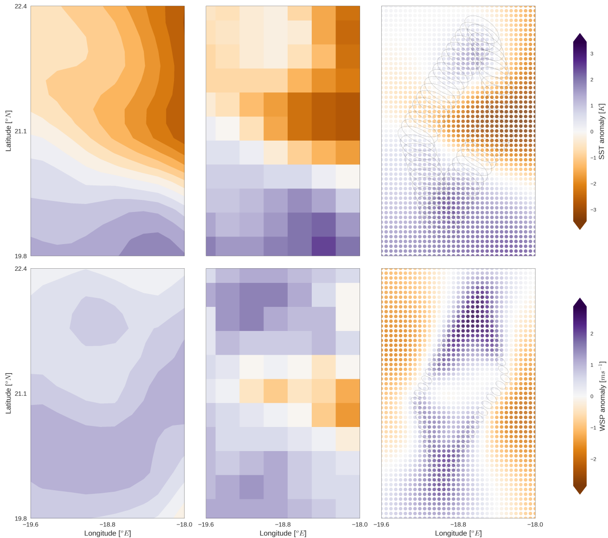
Figure 7. For the same scene as Fig. 6, the retrieved state vectors (right panels) are compared for SST (top row) and WSP (bottom row) against ERA5 (left) and RSS (middle). Each is displayed as the anomaly from the mean of the entire field. In the right panels, FOVs for the 6 and 36 GHz channels are shown for the pixels defining the edge of the observation area.
