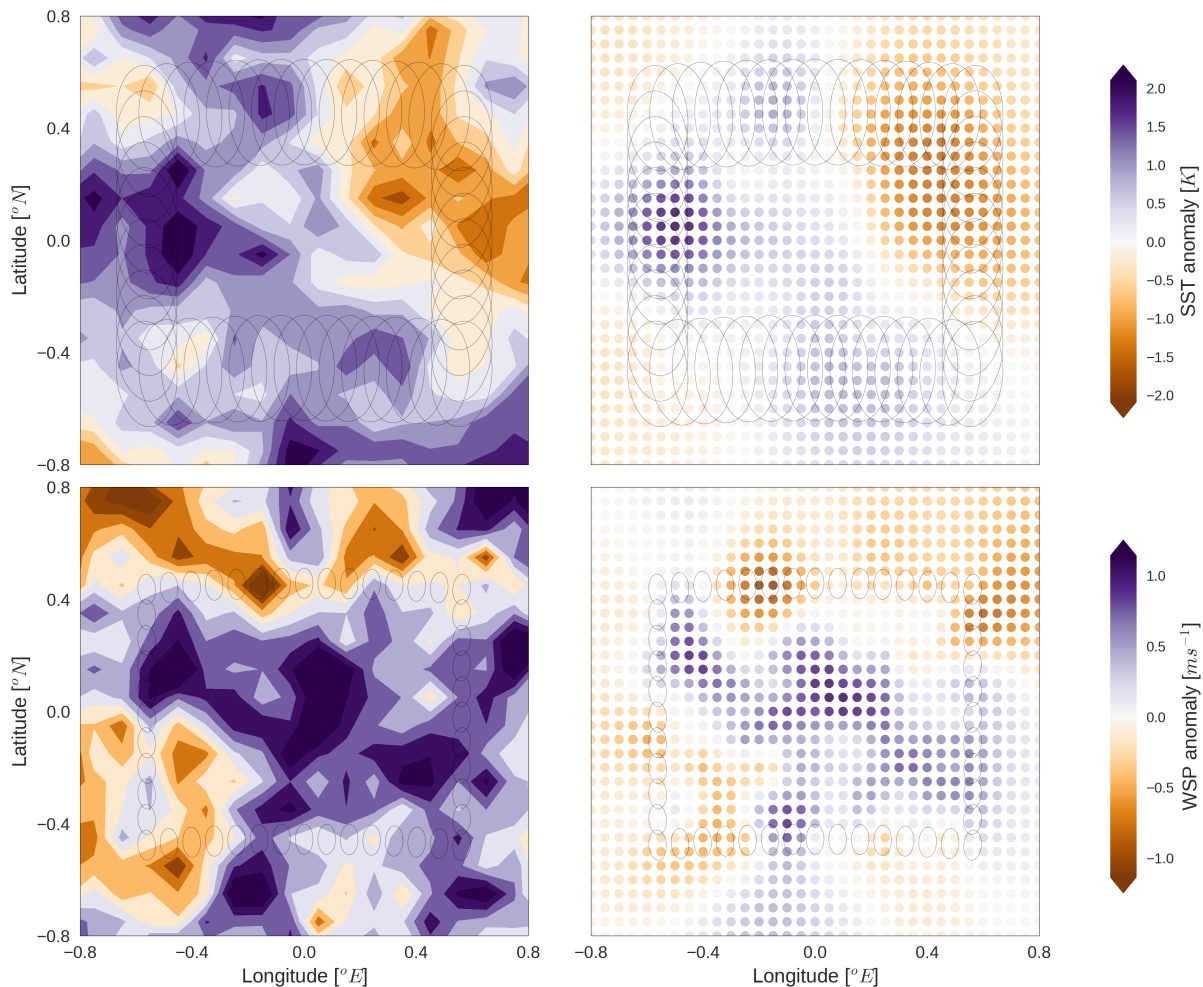
Figure 3. For the synthetic retrieval scene shown in contours (left panels), the retrieved state vectors are shown for SST (right top) and WSP (right bottom). Each dot represents a retrieval grid point. The fields are displayed as the anomaly from each field’s mean. FOVs for the 6 and 36 GHz channels are shown for the pixels defining the edge of the observation area.
