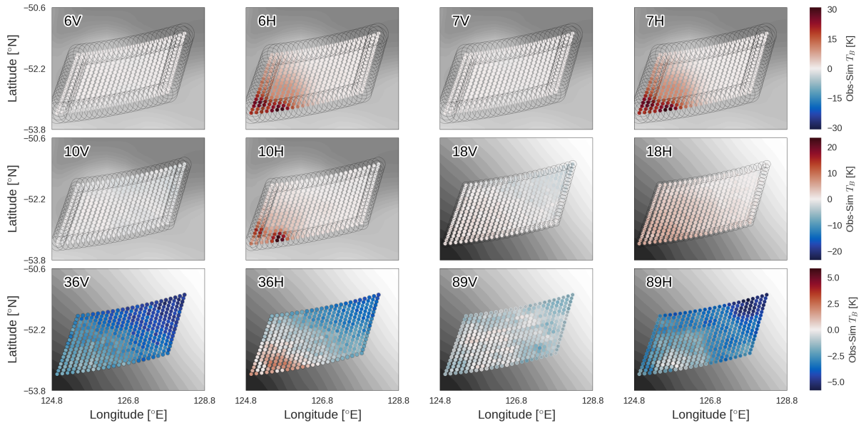
Figure 8. Observed minus simulated T_B for 12 AMSR2 channels after completion of the 2D-Var retrieval, south of Australia in the Southern Ocean on September 21, 2016. The background shows SST in the first six panels and WSP in the last six, with darker colours indicating higher values. Pixels on the edge of the measurement space are plotted along with their respective FOVs.
