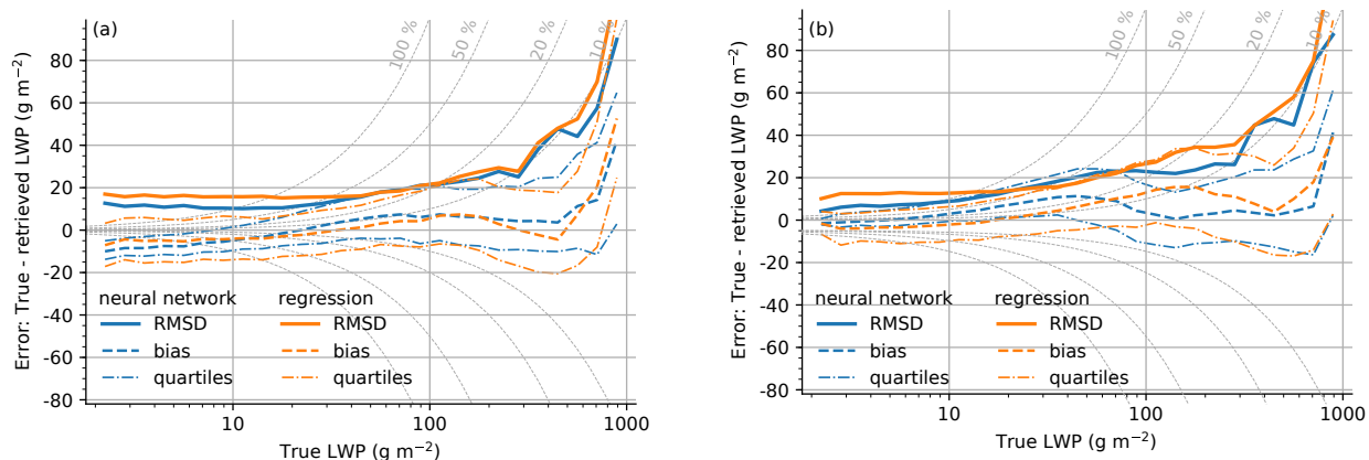
Figure 6. Expected retrieval error as function of true LWP for neural network and linear regression LWP retrievals. Retrievals (a) trained for 1 \text{ g m}^{-2} < LWP < 1000 \text{ g m}^{-2} . Retrievals (b) trained including clear sky cases ( LWP < 1000 \text{ g m}^{-2} ). Error measures (colored lines) for logarithmically distributed bins with ten bins per LWP power of ten. Gray dashed lines denote the corresponding relative LWP error.
