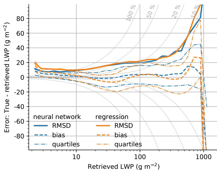
Figure 7. As Fig. 6, but with errors shown as function of retrieved LWP. Retrievals are trained and tested with 1 \text{ g m}^{-2} < LWP < 1000 \text{ g m}^{-2} . First bin contains all data with retrieved LWP < 2.5 \text{ g m}^{-2} (including negative).
